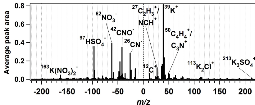
Fig. 4. A-TOFMS average mass spectrum of 52 fresh biomass burning particles sampled during RF03 plume Period 1.
