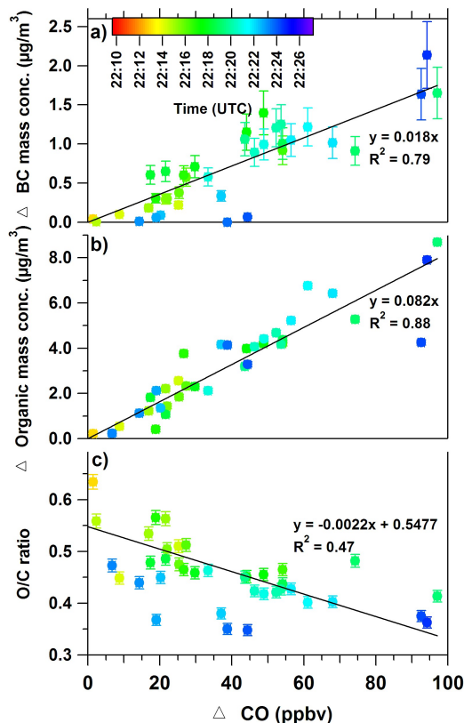
Fig. 6. Excess ( \Delta ) (a) SP2 black carbon (BC) mass concentrations and (b) C-ToF-AMS organic mass concentrations versus \Delta \text{CO} concentrations as a function of RF03 plume sample time. (c) C-ToF-AMS organic O/C ratio versus \Delta \text{CO} as a function of RF03 plume sample time. Note that CO data were not available over the entire RF03 smoke plume (see Fig. 2).
