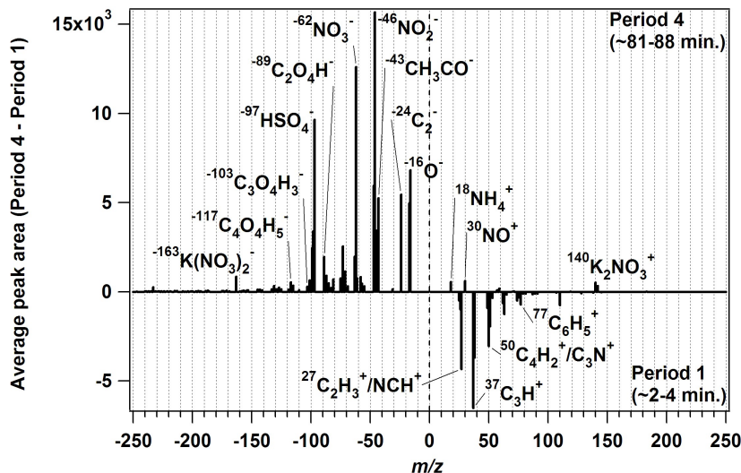
Fig. 5. A-ATOFMS average positive and negative ion mass spectra for biomass burning particles during RF03 Period 1 (age \sim 2 –4 min) subtracted from biomass burning particles during RF03 Period 4 (age \sim 81 –88 min). Positive intensity ion peaks indicate species added during aging of the individual biomass burning particles; negative intensity ion peaks indicate species with higher ion intensities within the fresh particles. Only ion peaks above 95% confidence limits following subtraction are shown.
