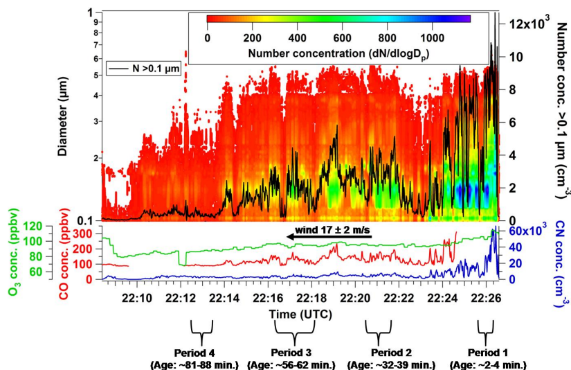
Fig. 2. RF03 temporal profiles of UHSAS size-resolved particle number concentrations with associated CO, O 3 , CN, and particles >0.1 μm concentrations are illustrated. Since CO data are not available for sampling closest to the burn source, maximum concentrations are estimated to be greater than the highest measured value of 311 ppbv, well above the average background air concentration of 92.6±0.9 ppbv. Aircraft was flying into the wind, as indicated by the arrow; therefore, later sampling times correspond to sampling closer to the fire source. Discussed time periods and calculated smoke plume ages are noted.
