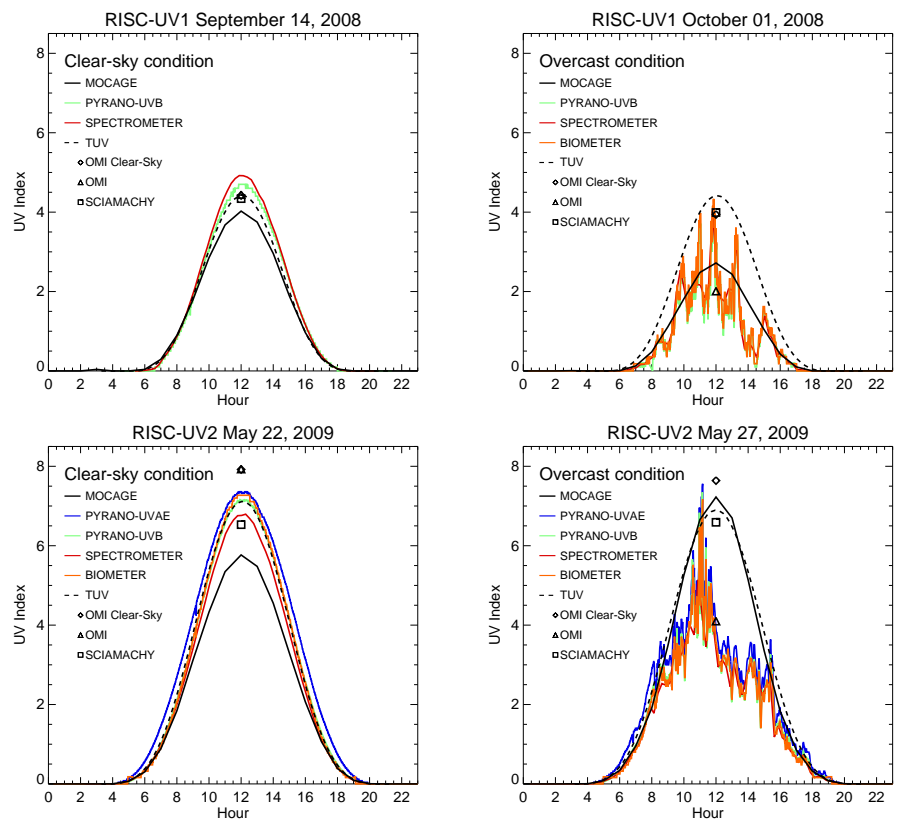
Fig. 4. Daily evolution of the UV index in clear-sky (left) and overcast (right) conditions during the RISC-UV campaign 2008 (top) and 2009 (bottom). MOCAGE simulation is compared to the SIRTa instruments (PYRANOMETER UVAE, PYRANOMETER UVB, SPECTROMETER, BIOMETER) and to the noon UV index values observed by the OMI (clear-sky and all-sky data), GOME2 (all-sky data) and SCIAMACHY (clear-sky data) instruments.
