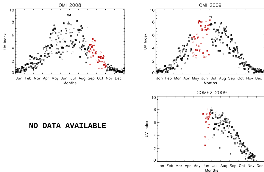
Fig. 3. OMI and GOME2 (all-sky data) satellite 2008 (left) and 2009 (right) UVI products. Red squares: RISC UV campaign periods.
