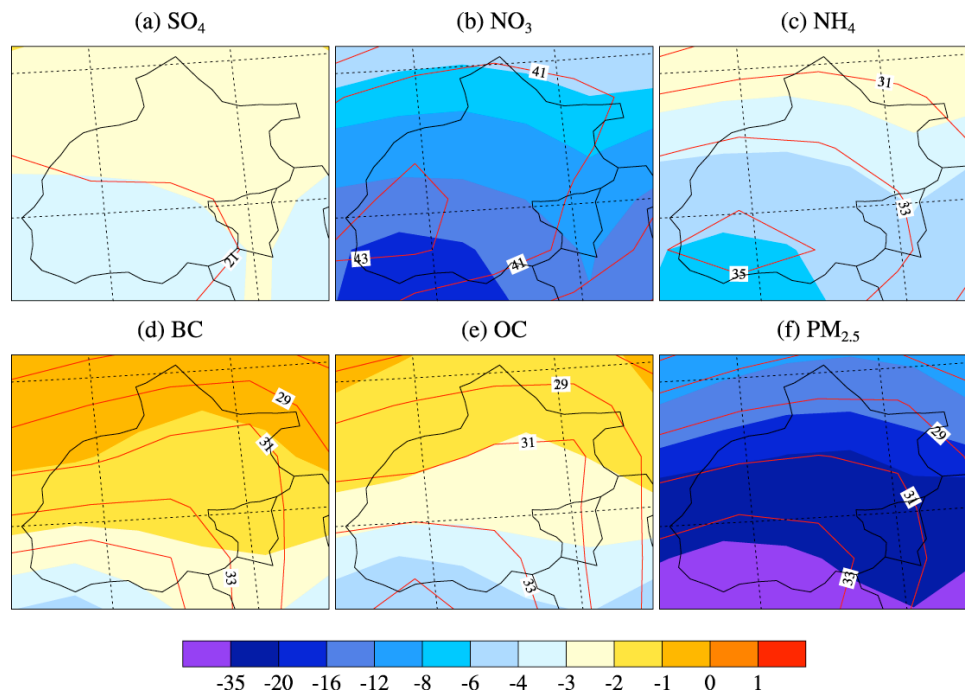
Fig. 3. Spatial distribution of the difference of time-averaged concentration between CTL case and NO-CTL case for (a) \text{SO}_4 , (b) \text{NO}_3 , (c) \text{NH}_4 , (d) BC, (e) OC, and (f) \text{PM}_{2.5} from 20 July to 31 August over Beijing. The color fill is the absolute difference in \mu\text{g m}^{-3} and the red solid contour lines with number are the relative differences in percentage (%).
