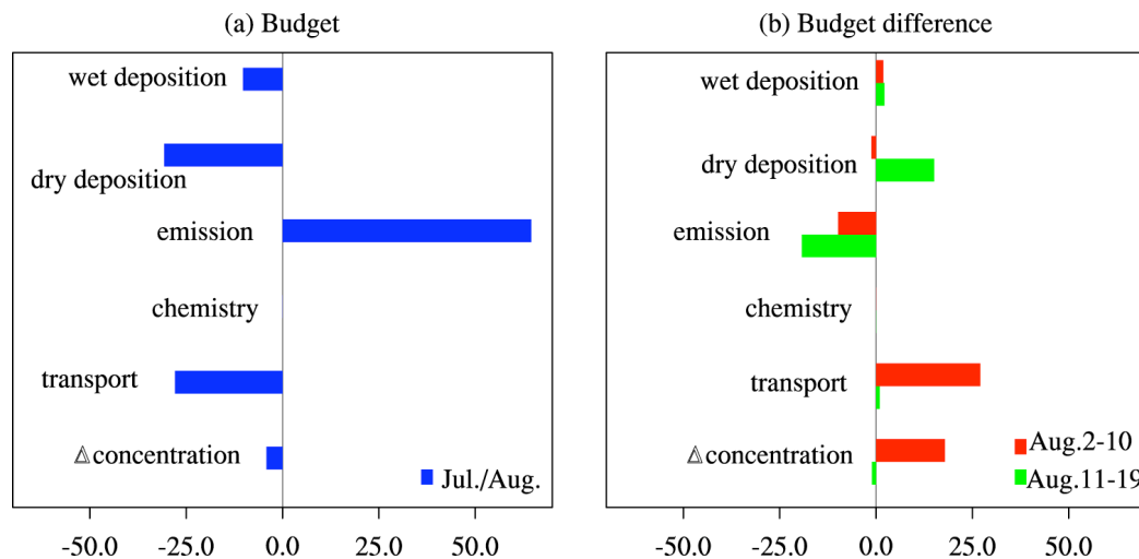
Fig. 6. (a) Budgets in July–August 2008 and (b) budget differences of the period 2 ~ 10 August (red) and 11 ~ 19 August (green) with July–August (blue) for BC over Beijing. \Delta concentration denotes variation of concentration. The positive value denotes increase to concentration and the negative value denotes decrease to concentration over Beijing. Unit: ton day -1 .
