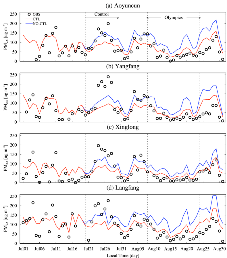
Fig. 2. Daily PM_{2.5} from observations and the corresponding WRF-Chem simulations in CTL and NO-CTL cases from 1 July to 31 August at the four sites (Aoyuncun, Yangfang, Xinglong and Langfang).
