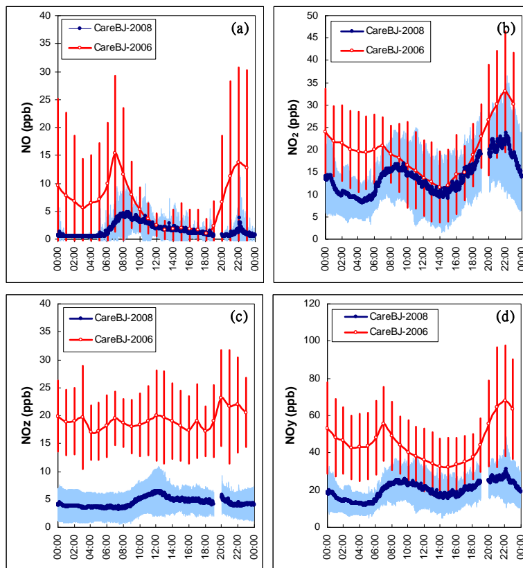
Fig. 2. Averaged diurnal variations in the mixing ratios of trace gases measured at the PKU observatory during the CAREBeijing-2006 and CAREBeijing-2008, respectively. The time resolution of the measurements, except NMHCs, of the 2008 campaign is 1 min, whereas the results of the 2006 campaign are hourly based. The ranges of \pm 1\sigma are indicated by the error bars associated with the hourly means or shaded for the 1-min. data. (a) NO; (b) NO 2 ; (c) NO z ; (d) NO y ; (e) CO; (f) NMHCs; (g) O 3 ; (h) O x .
