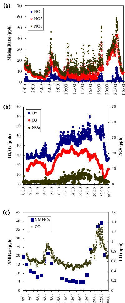
Fig. 7. Same as Fig. 3 but for 15 August 2008.
