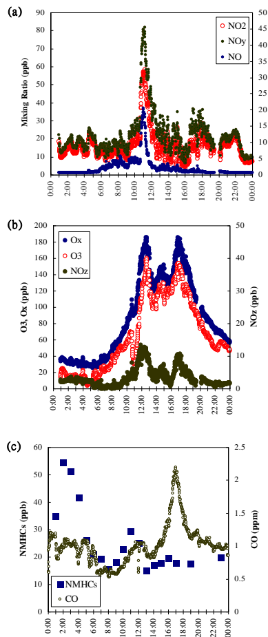
Fig. 3. Time series of the mixing ratios of trace gases and the meteorological conditions in Beijing for 3 August 2008. (a) NO, NO 2 , and NO y ; (b) O x , O 3 , and NO z ; (c) NMHCs and CO; (d) wind speed and direction; (e) ambient temperature, RH, and SWI.
