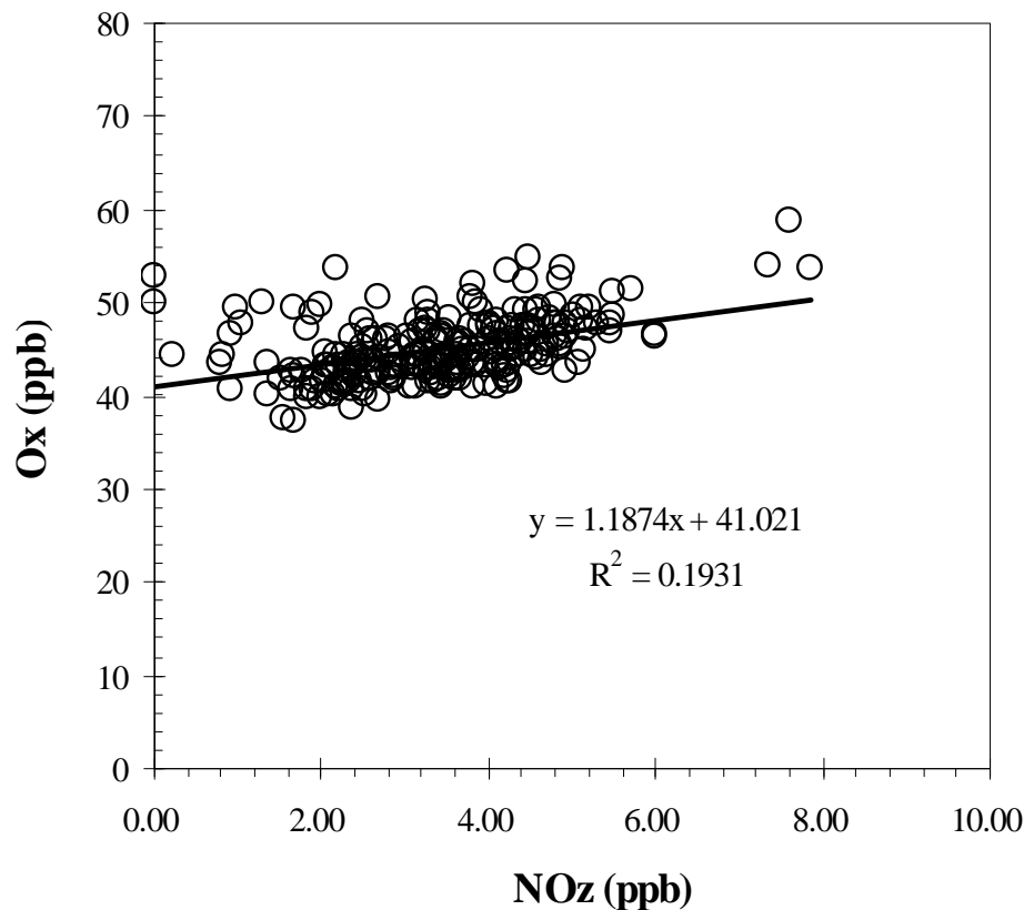
Fig. 8. Correlation between O x and NO z observed at the PKU observatory during the midday (10:00–14:00) of 15 August 2008. An averaged OPE x of 1.2 mole mole -1 is derived from the linear regression model.
