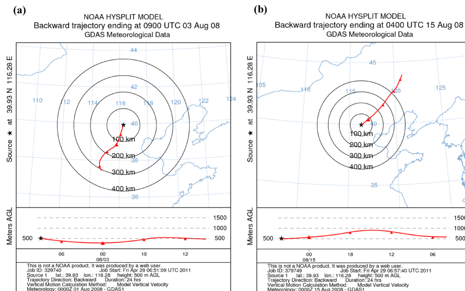
Fig. 6. Backward trajectories of air mass arriving Beijing at 17:00, 3 August (a) , and at 12:00, 15 August 2008 (b) . The trajectories were calculated for 24 h from an altitude of 500 m above the ground level of Beijing.
