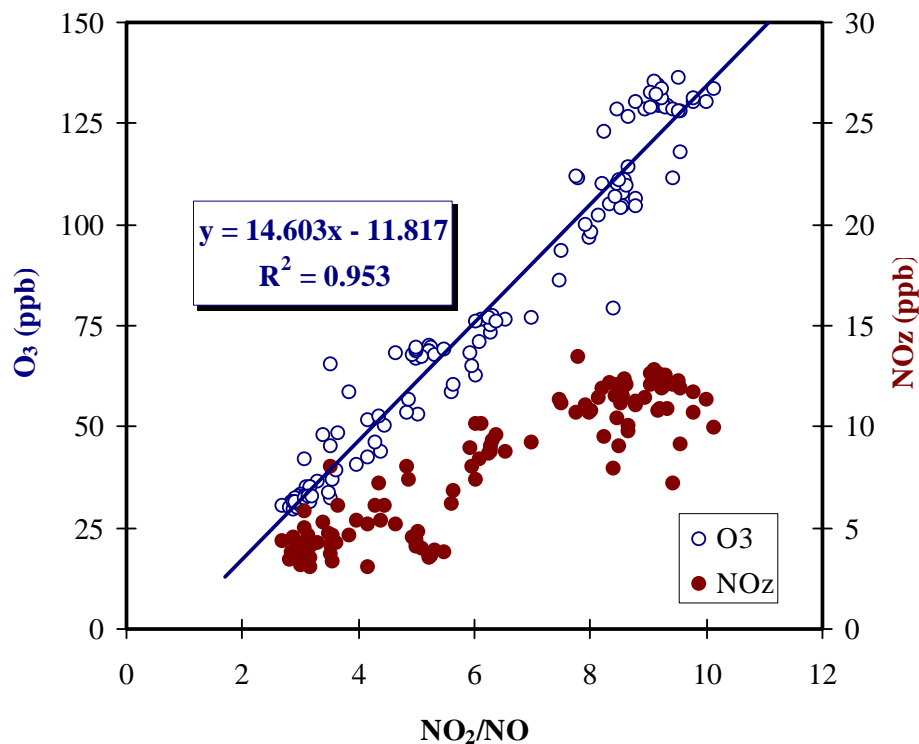
Fig. 5. Correlation of \text{O}_3 and \text{NOz} , respectively, versus the \text{NO}_2/\text{NO} ratio for the period of 10:30–12:30, 3 August 2008. The linear regression is associated to the \text{O}_3 data. The increasing trend of \text{NOz} with the \text{NO}_2/\text{NO} ratio is discontinued as \text{NO}_2/\text{NO} > 8 .
