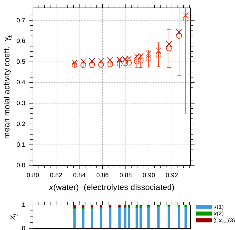
Fig. 7. Mean molal activity coefficients \gamma_{\pm} of KCl in the system water (1) + ethanol (2) + KCl (3) at 298 K. Experimental values (X) derived from EMF measurements by Lopes et al. (1999), calculated \gamma_{\pm} values (O) and corresponding activity coefficient sensitivities (error bars) are with regard to the mixed solvent reference state definition.
