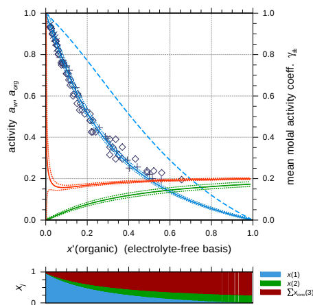
Fig. 11. Water activity measurements and AIOMFAC calculations for the system water (1) + malonic acid (2) + (\text{NH}_4)_2\text{SO}_4 (3). All mixtures are at a 1 : 1 molar ratio of malonic acid : (\text{NH}_4)_2\text{SO}_4 . Experimental bulk data for a_w at 295 K (+) by Choi and Chan (2002), EDB data at 298 K (+) by Ling and Chan (2008), and micro-Raman data at 297 K (◇) by Yeung and Chan (2010). Calculated curves at 298 K: a_w (solid blue), a_{\text{org}} of malonic acid (solid green), \gamma_{\pm} of (\text{NH}_4)_2\text{SO}_4 (solid red), and a_w of salt-free mixture (dashed blue). The dotted curves bordering the solid curves in the corresponding colors represent AIOMFAC sensitivities with respect to x^{\text{tol}} = 0.01 .
