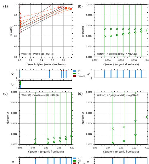
Fig. 13. Ternary systems containing multifunctional phenolic compounds. Experimental values are given by symbols (X) and respective AIOMFAC calculations by (O). (a) LLE of water (1) + phenol (2) + HCl (3) at 285 K. LLE composition measurements by Schreinemakers and van den Bos (1912). (b) Solubility limits of salicylic acid in aqueous KNO 3 solutions at 308 K. Measurements by Sugunan and Thomas (1995). (c) Solubility limits of vanillic acid in aqueous KCl solutions at 298 K. Measurements by Noubigh et al. (2007b). (d) Solubility limits of syringic acid in aqueous Na 2 SO 4 solutions at 298 K. Measurements by Noubigh et al. (2008).
