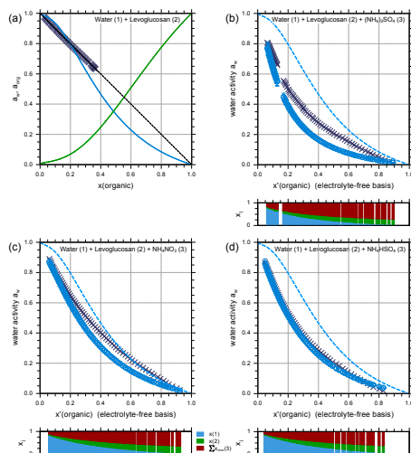
Fig. 14. Water activities of the binary and ternary water (1) + levoglucosan (2) + electrolyte (3) systems at 291 K. (a) In case of the binary system, the EDB water activity data (X) closely matches an ideal solution (dashed line). The AIOMFAC (UNIFAC) a_w -curve (blue line) shows larger deviations. The green curve shows the corresponding calculated activity of levoglucosan. (b) , (c) , and (d) Ternary systems containing the electrolytes ammonium sulfate, ammonium nitrate, and ammonium bisulfate, respectively, mixed at a molar ratio of 1 : 1 with levoglucosan. Symbols show the experimental water activity data (X) and corresponding AIOMFAC calculations (O). Error bars of the experimental data are smaller than the symbol size. The dashed, blue curve shows the electrolyte-free a_w model curve for comparison. Measurements by Lienhard et al. (2011).
