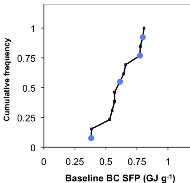
Fig. 1. Cumulative frequency distribution of global SFP from 13 models used in our paper (black line), compared with values from models proposed for use by reviewers (blue dots).
