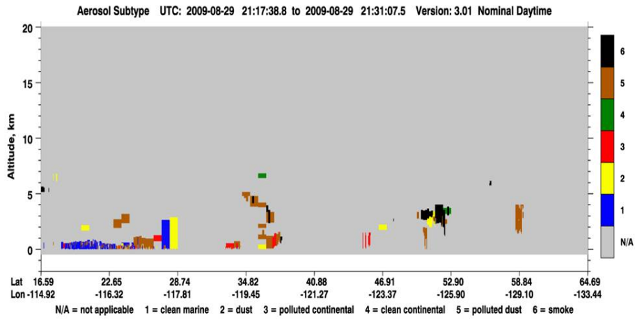
Fig. 2. CALIPSO overpass aerosol subtype product
