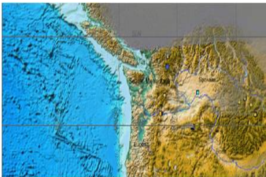
Fig. 1. Satellite smoke detection Aug 28-29 2009
