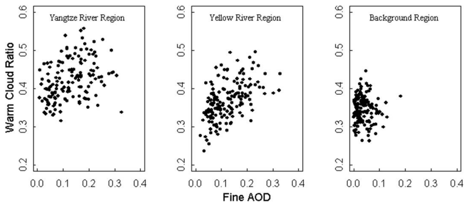
Fig. 4. Spatial correlation of fine mode AOD and warm cloud fraction.
