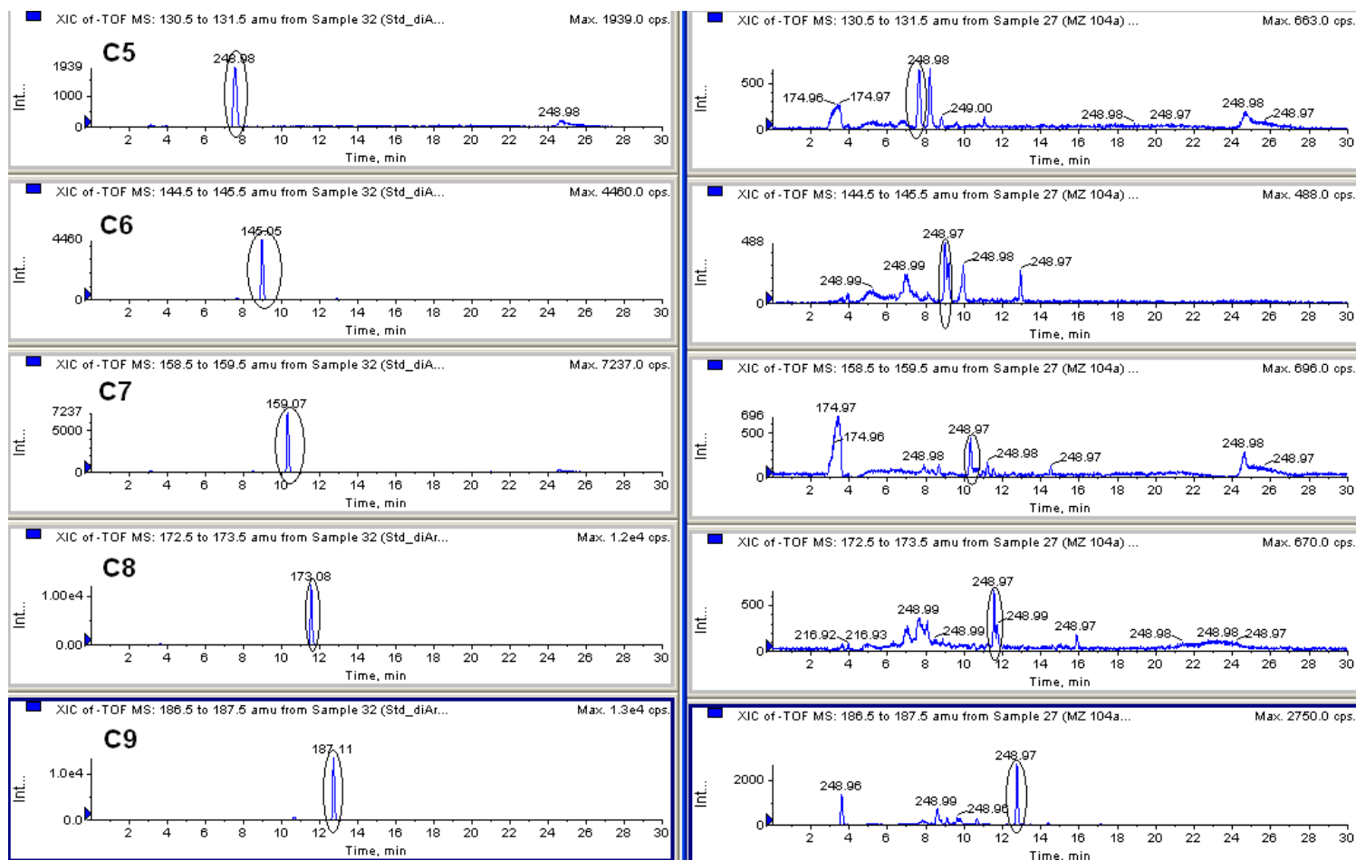
Figure S1 Typical extracted ion chromatograms of a standard (left) and aerosol particle samples (right).
