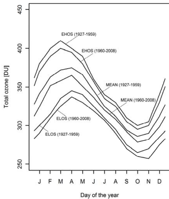
Figure 1: Daily thresholds for extreme high (EHOs) and low (ELOs) total ozone and interpolated mean values of total ozone over Arosa, for the periods 1927-59 and 1960-2008.
