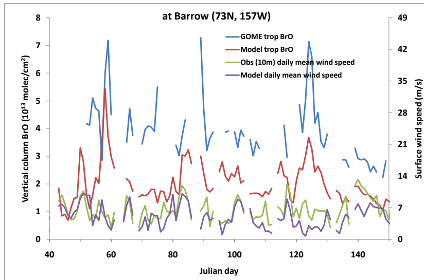
Fig. 1. supplementary figure 1: Observed 10 m daily mean wind speeds at Barrow airport (data from National Climatic Data Center) during Julian days 40-150, 1998, and model daily mean surface wind speeds.
