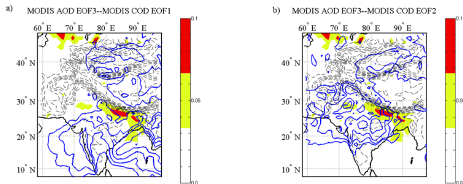
Fig. 2. Collocated plots of third mode of MODIS AOD (combined product of deep blue algorithm and dark target approach) and MODIS COD EOF 1 and EOF2. The contour of the MODIS COD is from 0.01 to 0.06 at an int
