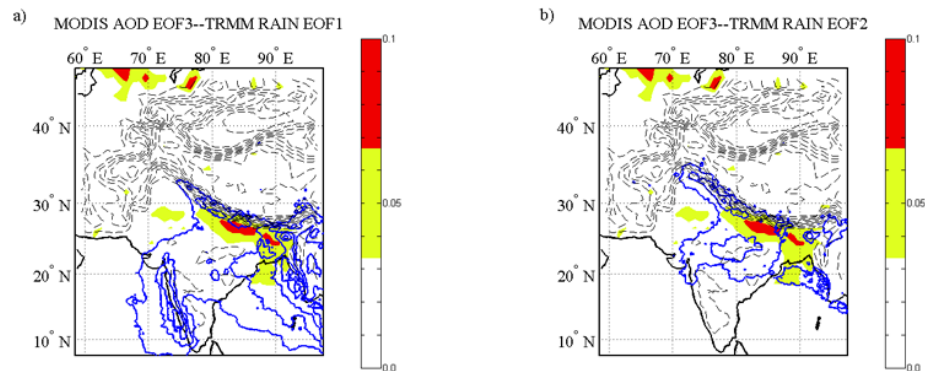
Fig. 1. Collocated plots of third mode of MODIS AOD (combined product of deep blue algorithm and dark target approach) and TRMM rainfall EOF 1 and EOF2. The contours of the TRMM rainfall EOFs are from 0.005
