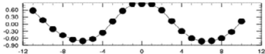
Fig. 6. Correlation between EC1 of MODIS AOD and TRMM rainfall with lag in the x-axis..
