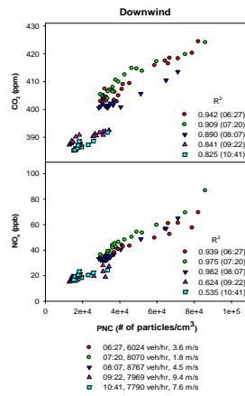
Figure B. Relationship between CO 2 and PNC and NO x and PNC measured downwind of I-93 throughout the morning on 16 January 2008.
