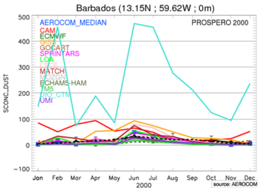
Fig. 1. Surface concentration for the year 2000 at Barbados
