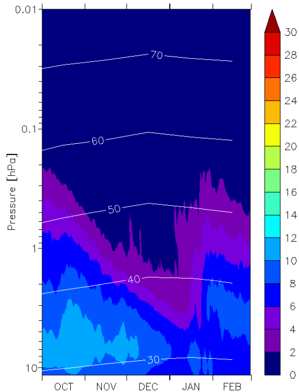
Fig. 1. NO x mixing ratio (ppbv) poleward of 60N in the simulation S-noEPP
