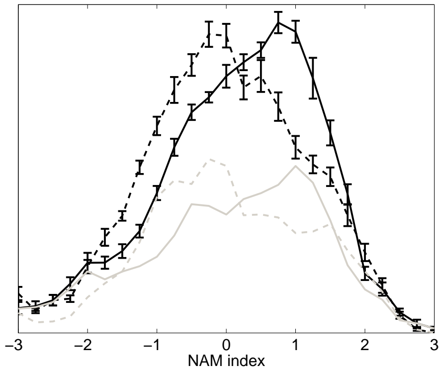
Fig. 3. Solid black: S-EPP, dashed black: S-noEPP. Error bars: standard deviation calculated from the individual years. Grey lines: analogous results for only those years where no SSWs occurred.
