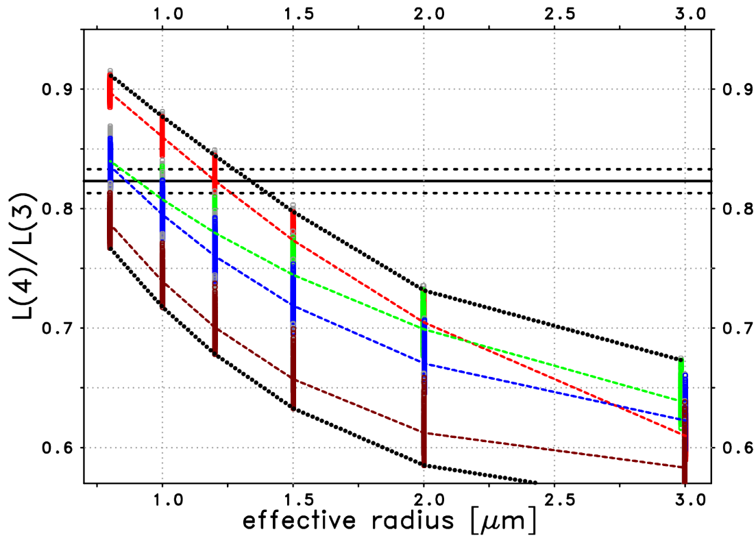
Fig. 1. Ratios of aureole radiances at 675nm (compare to Figure 9 of paper)
