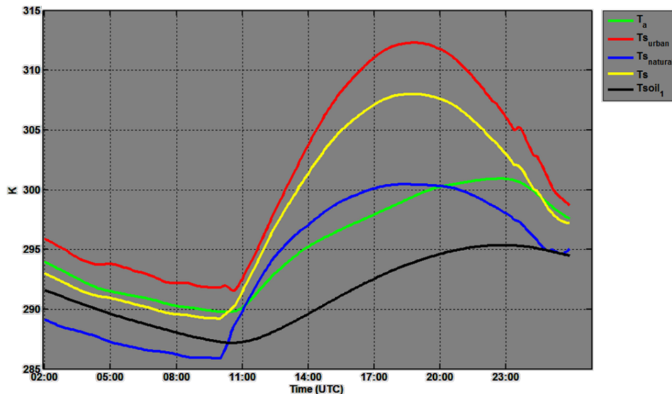
Figure R3: Change of temperature in time (UTC) for case 10s for the period 02Z 24 June – 01Z 25 June 2007 in units of K, including the lowest model layer temperature ( T_a ; ~ 28 m AGL here, green), the skin surface temperature over the urban canopy ( T_{s_{urban}} , red), the skin surface temperature over the natural surface ( T_{s_{natural}} , blue), the total skin surface temperature ( T_s , yellow) and the soil temperature of the upper-moist layer ( T_{soil_1} , black). Temperatures are averaged over all points in the fourth model layer except T_{s_{urban}} , which exists only in cells where f_{URB} > 0 .
