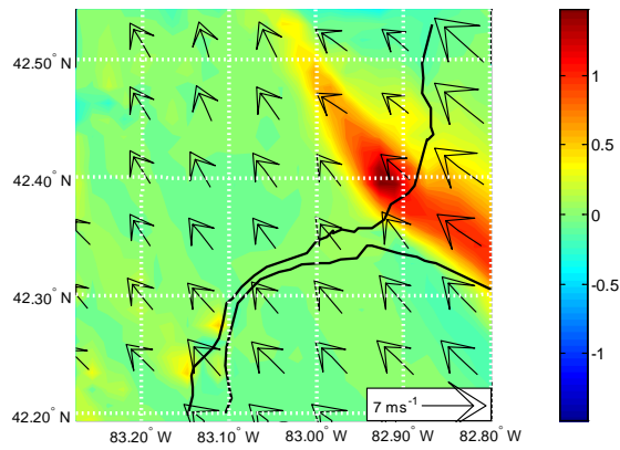
Figure R2: Temperature difference (case 10s – case 20s), (K), at the lowest model layer (~ 28 m AGL) over the third model grid of the domain at 23:20 UTC 24 June 2007. Horizontal wind speed for case 10s at this height is shown in black vectors scaled by the reference vector at the lower right.
