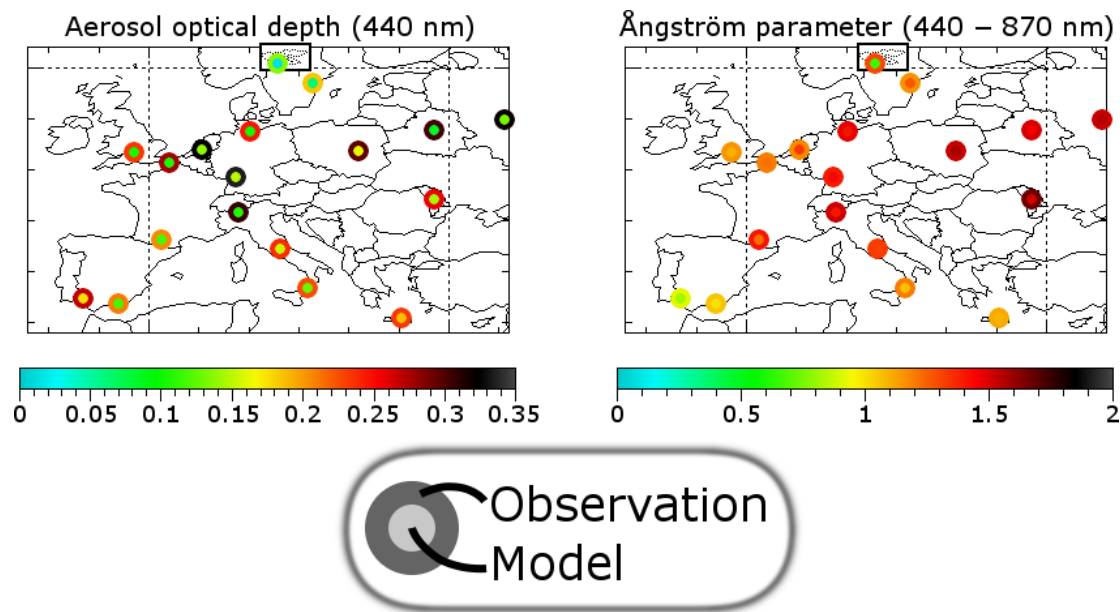
Fig. 2. Graphical overview of the comparison between modelled and observed AOD (440 nm) and Ångström parameter (440–870 nm). The country in the upper box is Svalbard (Norway).
