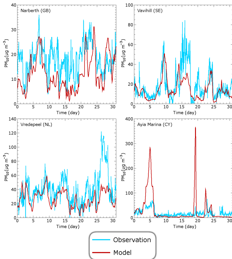
Fig. 3. Comparison between modelled and observed PM 10 concentrations of January 2006 for Narberth (GB), Vredepeel (NL), Vavihill (SE) and Ayia Marina (CY).
