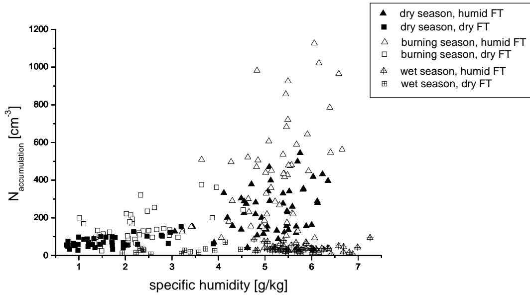
Figure 6: Relation between specific humidity and number concentration of accumulation mode particles.
