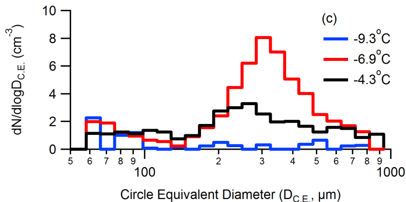
Fig. 1. Figure 12: Ice particle size distribution from the 2D-S in the convective region (15–25 km distance from CFARR) in (b) high ( >1 \text{ cm}^{-3} ) and (c) low ( <1 \text{ cm}^{-3} ) cloud droplet number concentration regions.
