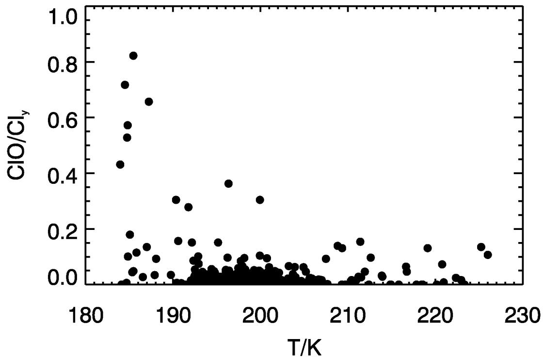
Fig. 1. \text{ClO}/\text{Cl}_y vs. Temperature
