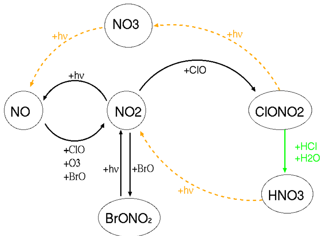
Fig. 2. The chemical reaction system governing NO x
