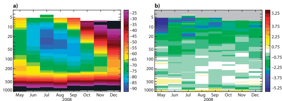
Fig. 4. Monthly mean of observed temperature profiles (left, in ^{\circ}\text{C} ) and respective forecast errors (right, in K) over Neumayer station for the period from May to December 2008.
