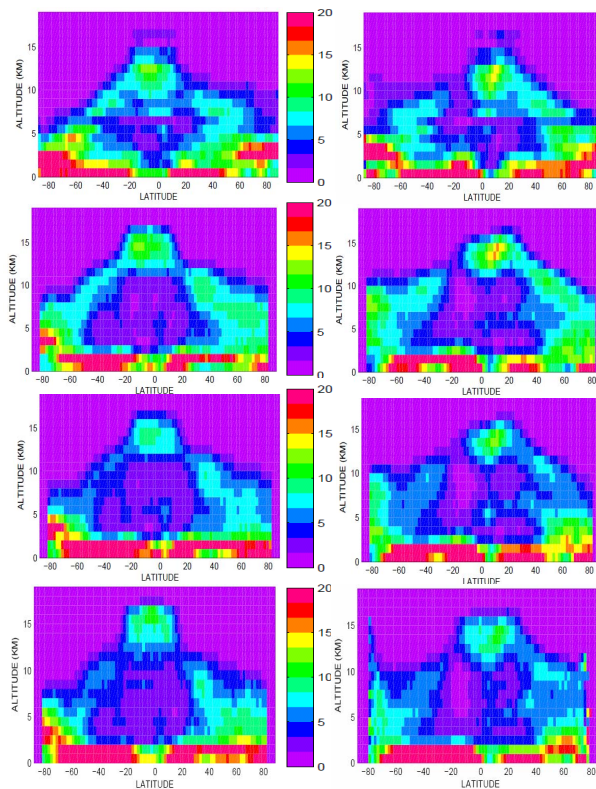
Fig. 8. Zonally averaged vertical distributions of relative cloud amount as obtained from AIRS-LMD (top panel), from CALIPSO (once for the uppermost cloud layer and once for all clouds detected at horizontal averaging of 5 km or less) and from Radar-Lidar GEOPROF (bottom panel), separately for boreal winter (left) and boreal summer (right). The data are normalized in such a way that the sum over all heights for each latitude interval corresponds to 100%. Averages over the period from 2007 to 2008.
