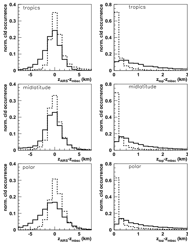
Fig. 5. Normalized frequency distributions of the difference between the cloud height of AIRS-LMD and the height of maximum backscatter of the uppermost cloud layer detected by CALIPSO at horizontal averaging over 5 km or less (left) and the difference between cloud top and height of maximum backscatter (right), separately for high clouds (full line) and mid-level/low clouds (broken line) as determined by CALIPSO, for the latitude bands 30° N–30° S (upper panels), 30°–60° (middle panels) and 60°–90° (lower panels).
