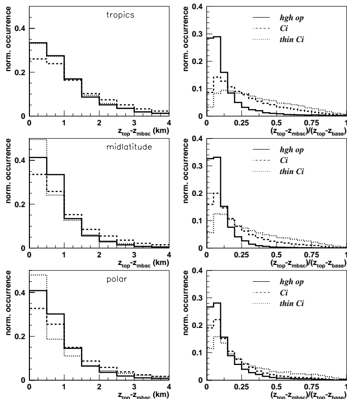
Fig. 9. Normalized frequency distributions of the height of maximum backscatter in relation to the cloud top, separately for high opaque clouds (full line), cirrus (broken line) and thin cirrus (dotted line), as absolute difference z_{\text{top}} - z_{\text{mbsc}} (left panel) and as relative difference (z_{\text{top}} - z_{\text{mbsc}})/(z_{\text{top}} - z_{\text{base}}) (right panel). Distributions are presented for three different latitude bands: 30^{\circ} N– 30^{\circ} S (upper panels), 30^{\circ} – 60^{\circ} (middle panels) and 60^{\circ} – 90^{\circ} (lower panels).
