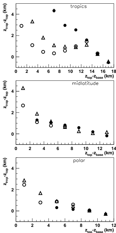
Fig. 14. Average difference between the height of the tropopause and the cloud top as a function of real cloud geometrical thickness, separately for high opaque clouds (full circles), cirrus (open triangles) and thin cirrus (open circles) and for three different latitude bands: 30^{\circ} N– 30^{\circ} S (upper panel), 30^{\circ} – 60^{\circ} (middle panel) and 60^{\circ} – 90^{\circ} (lower panel).
