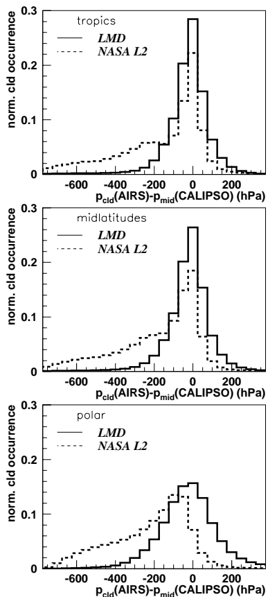
Fig. 4. Normalized frequency distributions of the difference between AIRS cloud pressure and pressure of the “apparent middle” of the uppermost cloud layer detected by CALIPSO at horizontal averaging over 5 km or less. Observations at 01:30 LT. AIRS cloud retrievals from LMD are compared to those of NASA L2 products, separately for the latitude bands 30° N–30° S (upper panel), 30°–60° (middle panel) and 60°–90° (lower panel).
