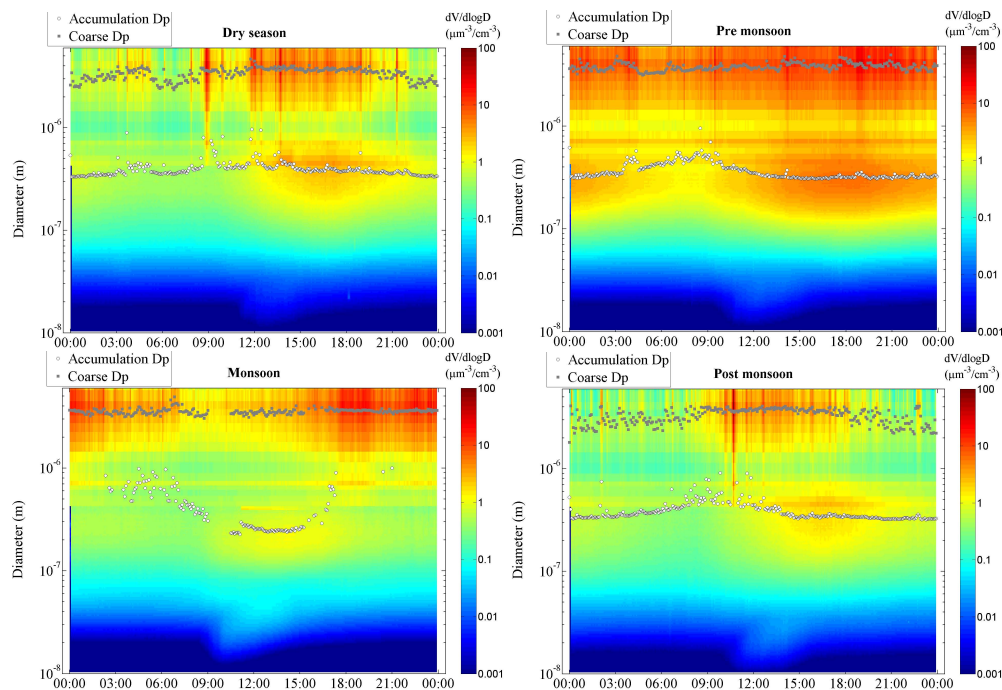
Fig. 2. Mean diurnal variation of the aerosol volume size distribution detected from 10 to 6000 nm and accumulation and coarse diameter mode fitted on aerosol volume size distribution, averaged over the whole measurement period for the (a) dry season, (b) pre-monsoon season, (c) monsoon season and (d) post-monsoon season.
