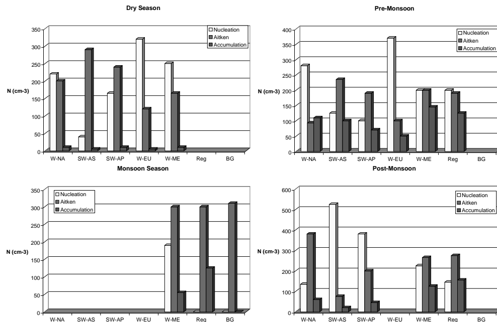
Fig. 3. Contribution of the nucleation, Aitken and accumulation modes integrated number concentrations to the total aerosol number concentration for different air mass types for the (a) dry season, (b) pre-monsoon season, (c) monsoon season and (d) post-monsoon season.
