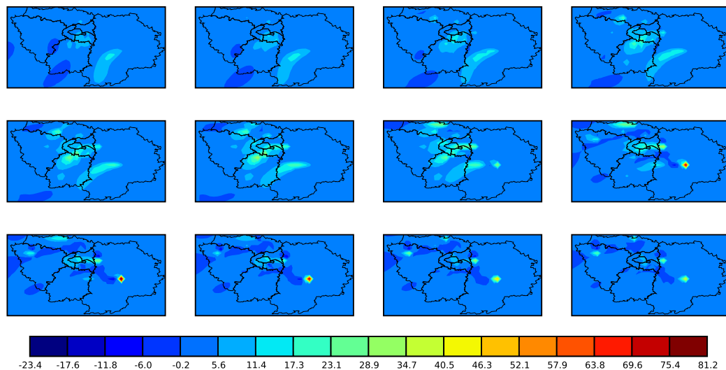
Fig. 9. Evolution of the difference between reference and plume-in-grid SO 2 ground concentrations during twelve hours, from 23 August at 03:00 (local hour) to 23 August at 14:00. Unit is µg m -3 . Plume-in-grid concentrations are subtracted to the reference concentrations.
