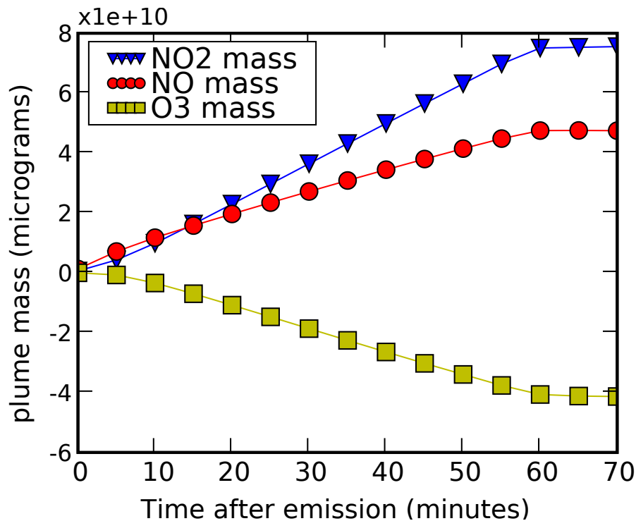
Fig. 2. Plume mass in \mu\text{g} for \text{NO}_2 , \text{NO} and \text{O}_3 with plume-in-grid. Simulation with one point source of \text{NO}_x in a uniform background of \text{O}_3 .
