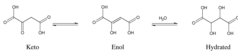
Fig. 2. The three forms of oxosuccinic acid in aqueous solution.
