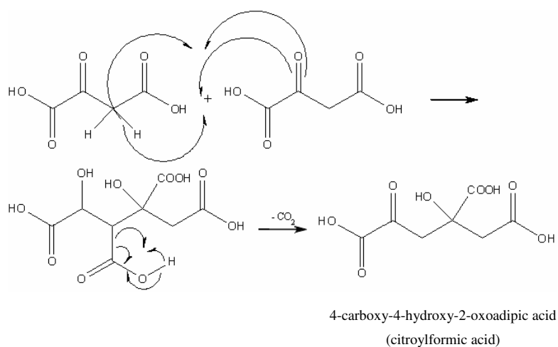
Fig. 4. Aldol reactions of oxosuccinic acid.
