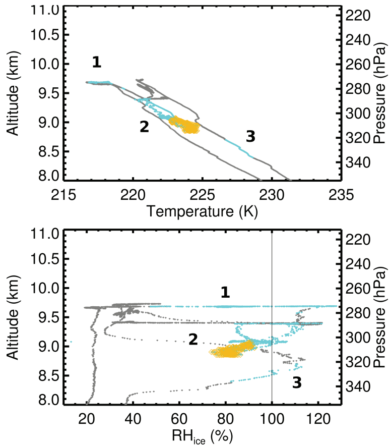
Fig. 5. Vertical profiles of cirrus (turquoise) and contrail (orange) temperature and RH_{ice} during the 1st flight on 17 November 2008. Cirrus periods 1: 11:40–11:55 UTC, 2: 12:10–12:40 UTC (including the A343 contrail) and 3: around 13:00 UTC.
