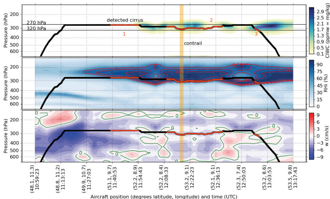
Fig. 7. Vertical cross sections of ECMWF analyzed cloud ice water content (CIWC), RH_{ice} and vertical velocity ( w ) on 17 November 2008, 12:00 UTC along the flight route. The in-situ detected cirrus periods are highlighted in orange on the flight profile. The contrail event is indicated by the orange bar.
