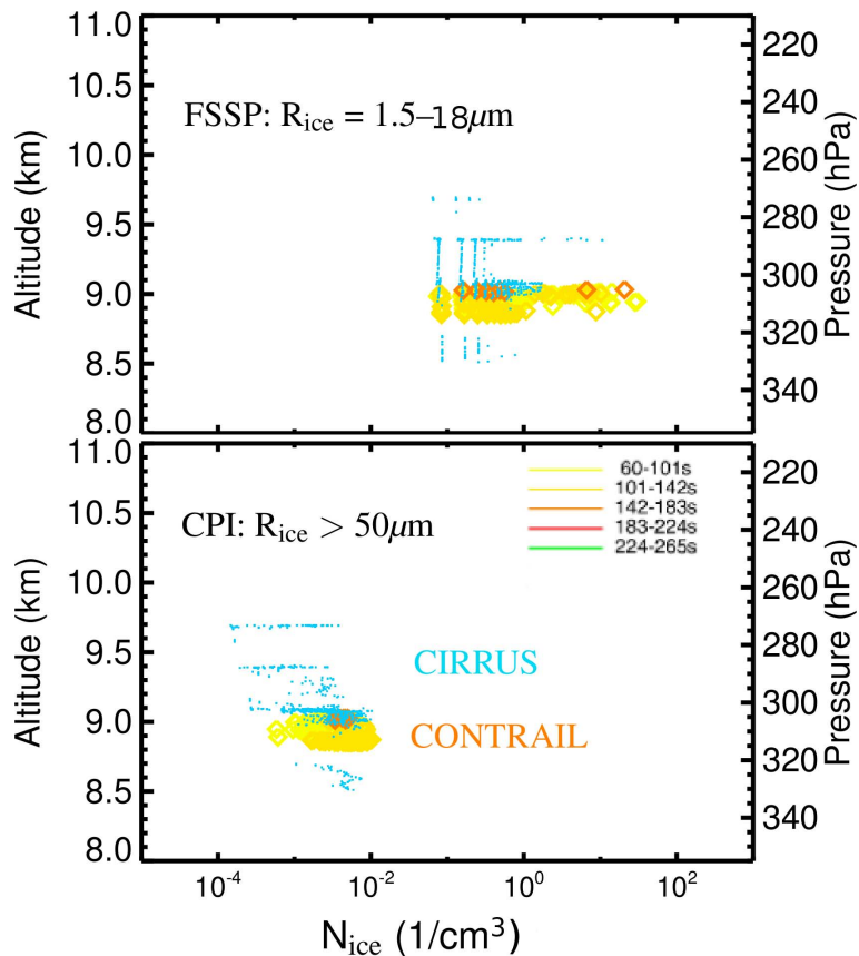
Fig. 6. Vertical profiles of the ice crystal number N_{ice} for different size intervals in the 2. cirrus (turquoise) period of the 1st flight on 17 November 2008, including the A343 contrail (coloured by age, see legend in bottom panel). Cloud particle instrumentation: FSSP – Forward Scattering Spectrometer Probe and CPI – Cloud Particle Imager, for more information see Sect. 2.
