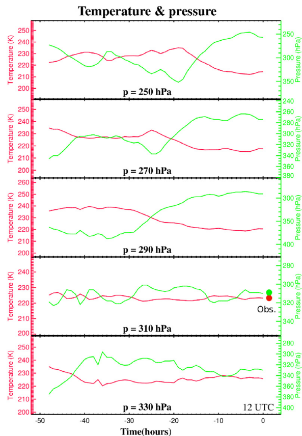
Fig. 9. Temperature and pressure along the trajectories shown in Fig. 8, ending at the point of contrail detection at 310 hPa. In the 310 hPa panel, big dots denotes the observations (see Figs. 4 and 5).
