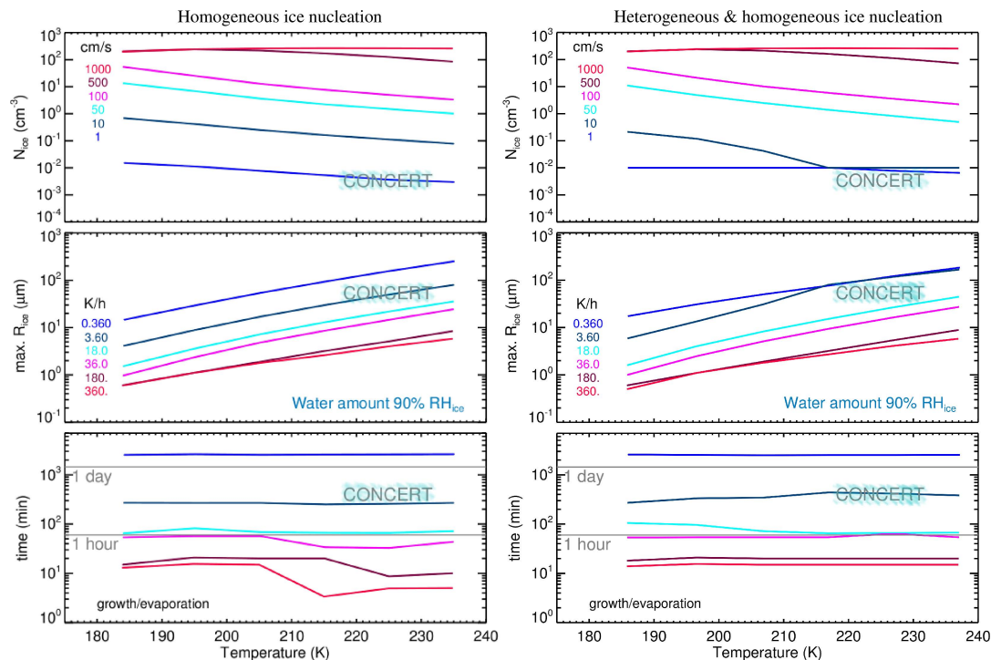
Fig. 11. Ice crystal number (top), maximum size (middle) and growth/evaporation times (bottom) in dependence on temperature and cooling rate ( \sim vertical velocity): idealized model simulations performed with MAID assuming pure homogeneous (left) and heterogeneous and homogeneous (right) freezing as ice nucleation mechanism (see also Krämer and Hildebrandt, 2010). The initial conditions of the model runs are as follows: pressure= f(T) (Schiller et al., 2008), particle number= 300 \text{ cm}^{-3} , mean particle radius 0.2 \mu\text{m} . The heating rates during evaporation correspond to the respective cooling rates. The range of observations during CONCERT are indicated in grey letters.
