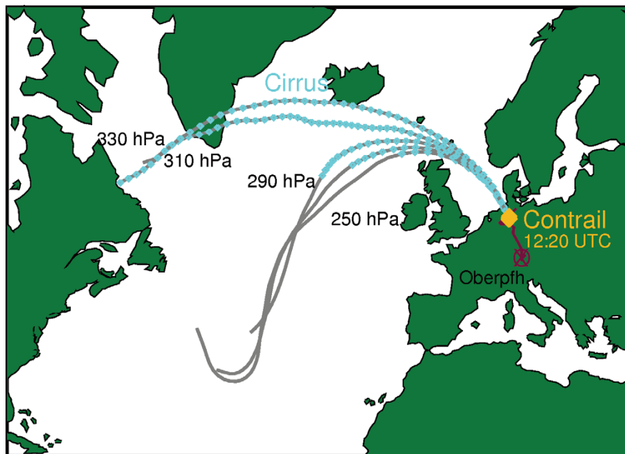
Fig. 8. ECMWF air mass trajectories in different pressure levels, starting approximately at the geographical coordinates of contrail detection on 17 November 2008; turquoise dots represent ECMWF ice.
