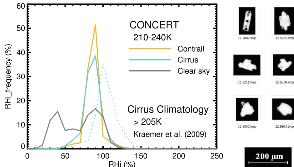
Fig. 2. Left panel: Frequency of occurrence of RH_{ice} in contrails, cirrus and clear sky during CONCERT (solid lines) and for a broad range of cirrus conditions (dotted line, from Krämer et al., 2009, 5.6 h observation time, 28 flights). CONCERT sampling times: clear sky 0.9 h, cirrus 2.3 h, contrails 1.7 h, flight dates: 29 October (1 flight), 17 November (2 flights), 19 November (2 flights), 20 November (1 flight). Right panel: large ice crystals observed inside of the cirrus and contrails during CONCERT.
