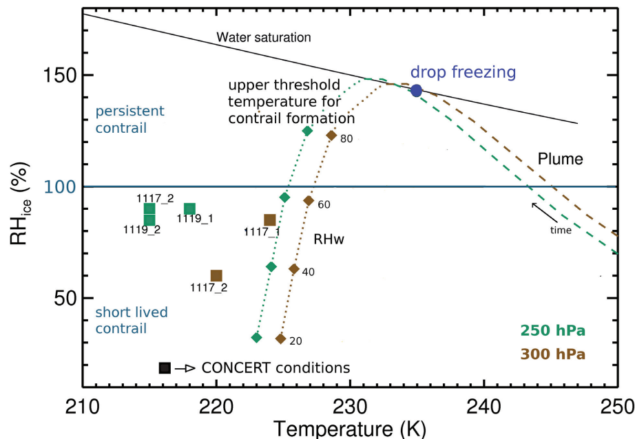
Fig. 1. Ambient temperature and humidity conditions during four CONCERT flights (rectangles, colored by pressure, labeled with mmdd.flightnumber) and calculated upper threshold temperatures for contrail formation for the same pressures and varying RH_w (relative humidity wrt water; dotted lines with diamonds): the contrail formation criterion was well fulfilled during the flights. Dashed lines: calculated evolution of aircraft plume temperatures and RH_{ice} until drop formation and freezing for the two mean ambient pressures.
