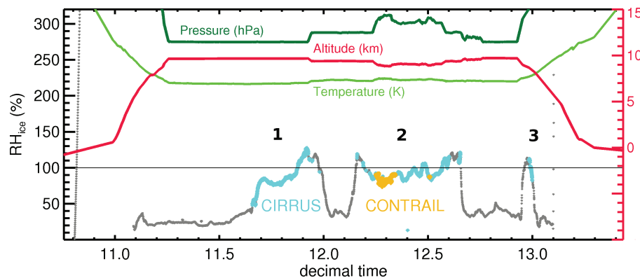
Fig. 4. Survey of DLR Falcon's 1st flight on 17 November 2008, 11:00 to 13:20 UTC. Top panel: flight path, turquoise/orange indicate cirrus/contrails. Bottom panel: temperature, pressure, altitude and RH_{ice} along the flight path. DLR Falcon crossed three cirrus sections, labeled 1–3 in the following.
