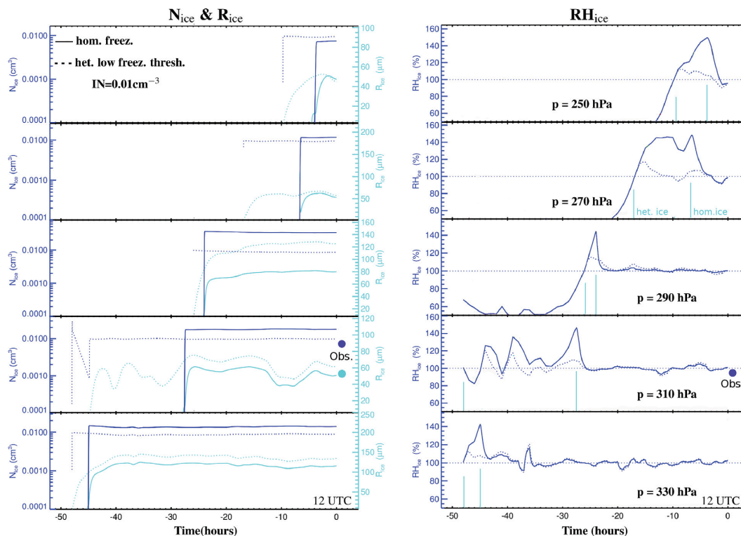
Fig. 10. MAID simulations along the trajectories shown in Figs. 8 and 9 (solid line: homogeneous freezing, dotted line: heterogeneous freezing); N_{\text{ice,MAID}} : number, R_{\text{ice,MAID}} : mean mass size of ice crystals. In the 310 hPa panels, big dots denotes the observations ( N_{\text{ice,obs}} : peak number, R_{\text{ice,obs}} : approximate size of ice crystals, see Fig. 6, bottom panel; \text{RH}_{\text{ice}} see Fig. 5).
