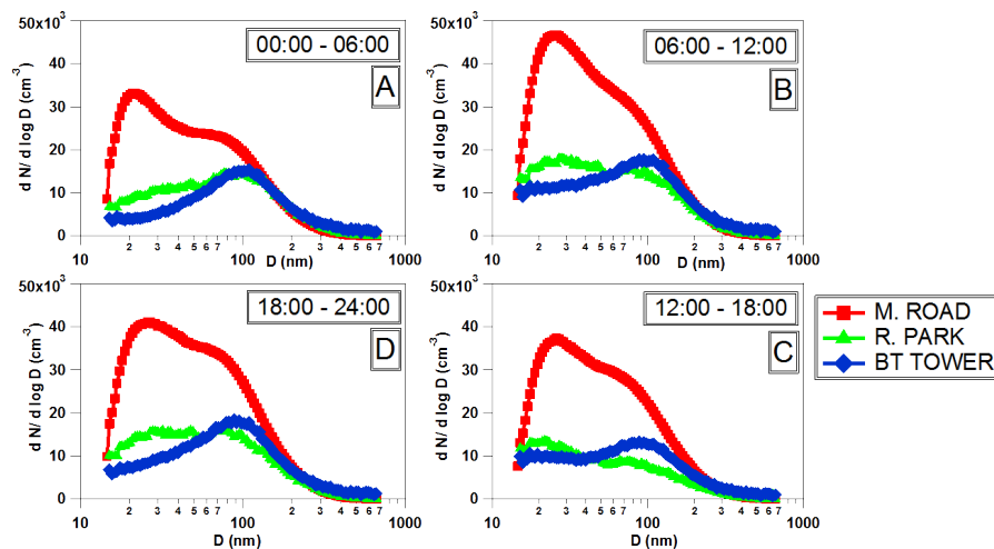
Fig. 5. Average SMPS size distributions for 3 different sites (MR, R. Park and BT Tower) taken simultaneously during the REPARTEE-II field study. Data are average for the 6 h time period at 00:00–06:00 (A), 06:00–12:00 (B), 12:00–18:00 (C) and 18:00–24:00 (D).
