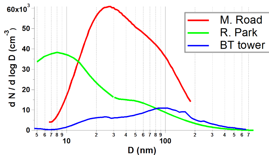
Fig. 3. Average particle size distributions (mobility diameter, nm) at Marylebone Road, Regents Park and BT Tower.
