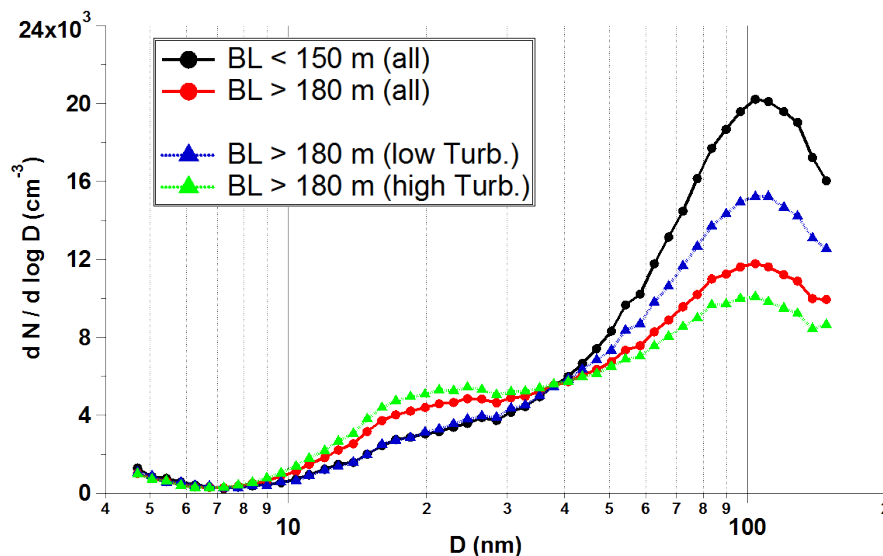
Fig. 7. Average nano-SMPS size distributions at the BT Tower site (BT Tower) for periods of: UBL height below the BT Tower tower sampling height (<150 m); high UBL height (>180 m); low \sigma_w^2 (<0.5 m 2 s -2 ) and high \sigma_w^2 (>0.5 m 2 s -2 ). Measurements of UBL height and \sigma_w^2 were derived from the Lidar.
