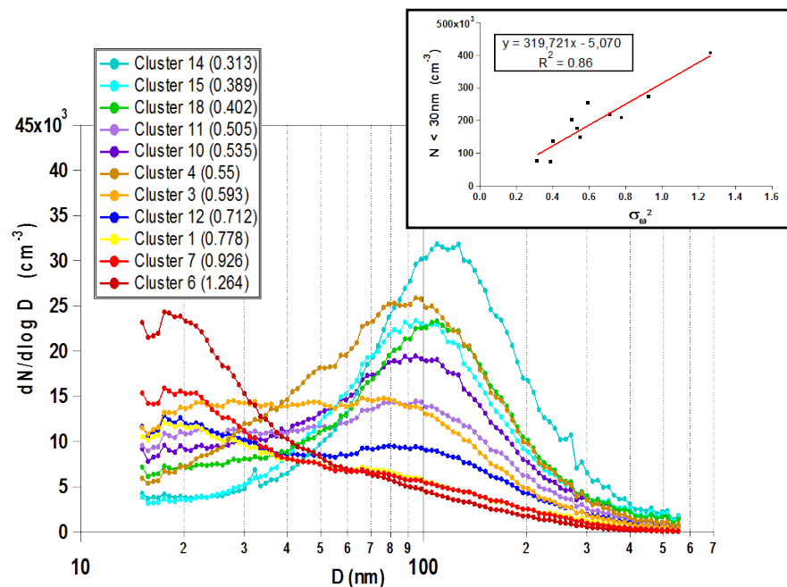
Fig. 8. SMPS cluster analysis from the BT Tower site. For each of the 11 clusters reported, in the legend an average value of \sigma_w^2 ( \text{m}^2 \text{s}^{-2} ) obtained with the Lidar is given.
