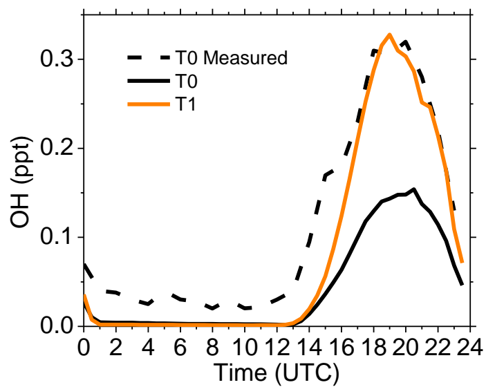
Figure S1: Comparison of measured vs. WRF-Chem predicted 24-day average diurnal variation of OH concentration at T0 site in Mexico City. Predicted diurnal variation of OH at T1 site is also included for comparison.
