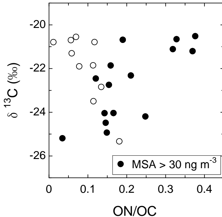
Fig. 6. Scatter plots between \delta^{13}\text{C} and ON/OC ratios. Solid circles indicate the data with MSA > 30 ng m -3 .
