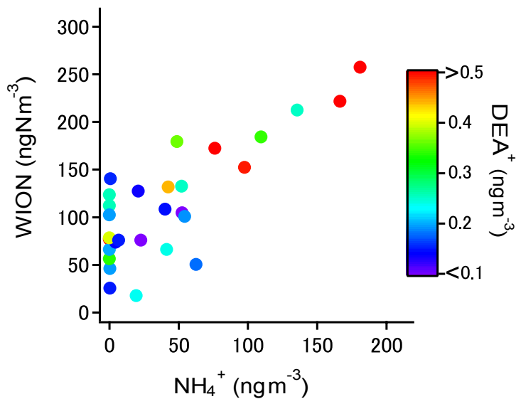
Fig. 8. A linear relation between WION and NH 4 + , color-coded according to the concentration of DEA + .
