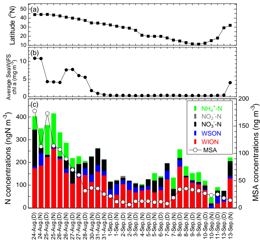
Fig. 3. Time series of (a) the average latitudinal location of the ship, (b) concentrations of trajectory-weighted chlorophyll a and (c) fractions of organic (WSON and WION) and inorganic nitrogen together with concentrations of MSA. “D” means data obtained in daytime, whereas “N” means data obtained in nighttime.
