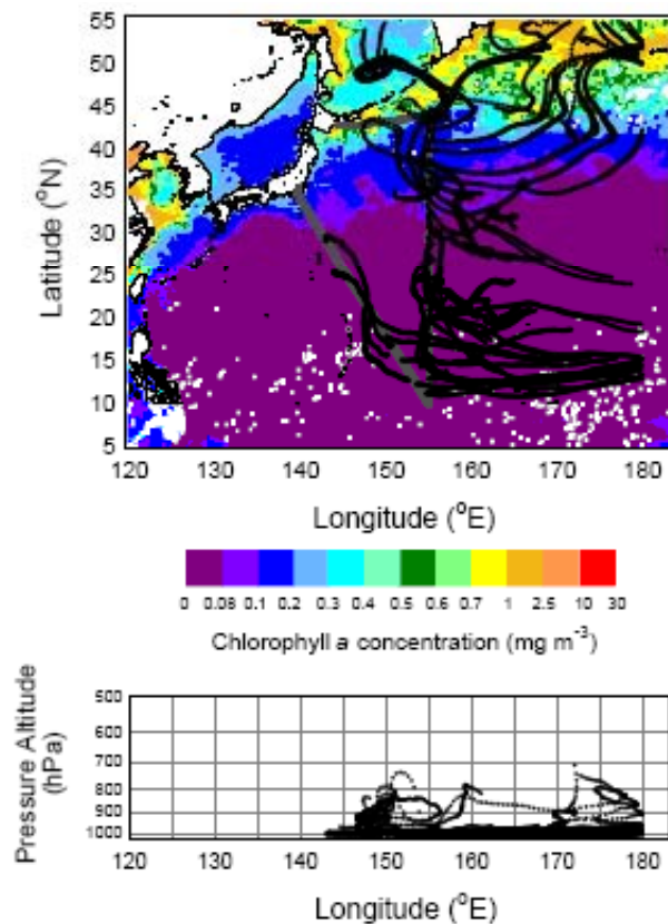
Fig. 1. R/V Hakuho cruise track in the western North Pacific between 24 August and 13 September 2008, together with typical 5-day back trajectories. Also shown are monthly averaged concentrations of chlorophyll a for August–September 2008 derived from SeaWiFS data, available from the NASA Goddard Space Flight Center/Distributed Active Archive Centers. A white dot indicates that the satellite data is missing at a corresponding grid.
