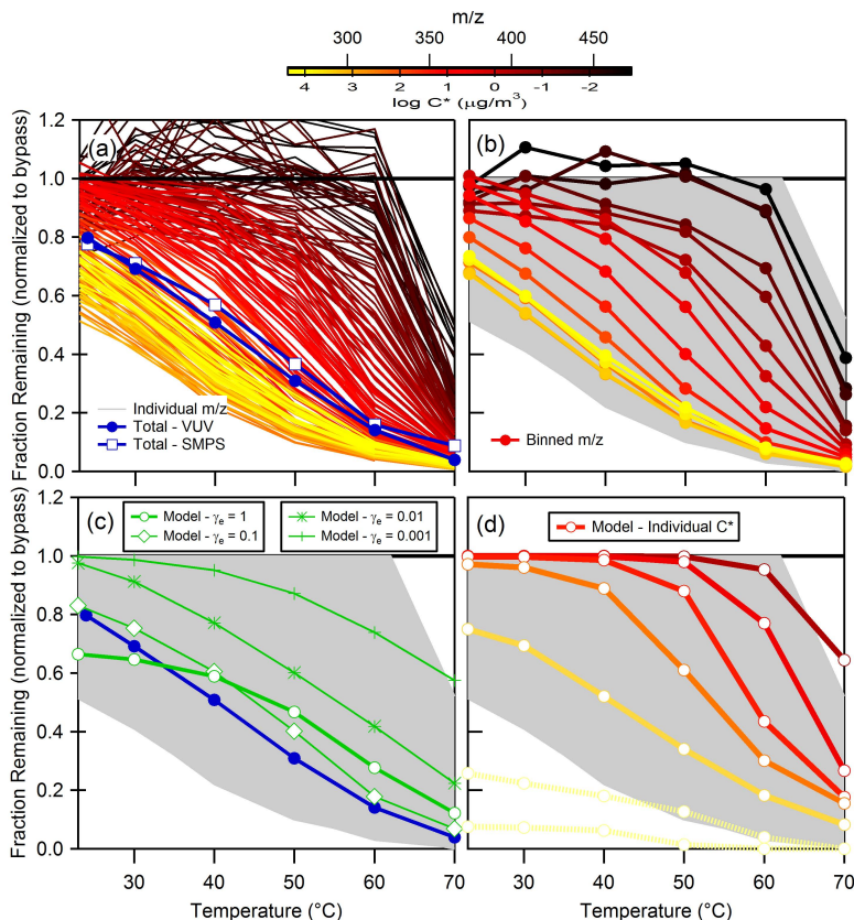
Fig. 3. (a) Total mass thermograms (blue) from SMPS (open squares) and VUV intensity (filled circles) measurements and peak thermograms for every m/z from m/z = 260 to 477 amu (thin lines) for LO particles. Line colors indicate the m/z (see color scale). (b) Same as (a), but where the results from the individual peaks have been binned into narrower mass ranges to illustrate the m/z dependence. (c) Calculated total mass thermograms for model LO aerosol for different values of \gamma_e (green). The measured value is shown for reference (blue). (d) Calculated mass thermograms for each model LO component (i.e. different C^* ) are shown, assuming \gamma_e = 0.5 . Line colors correspond to the C^* values and range from 10^{-2} to 10^4 \mu\text{g}/\text{m}^3 . Note that the C^* = 10^3 and 10^4 \mu\text{g}/\text{m}^3 components are above the color scale and shown as faded to indicate this. The gray region in panels b, c and d indicates the range over which individual m/z peak thermograms in (a) were observed.
