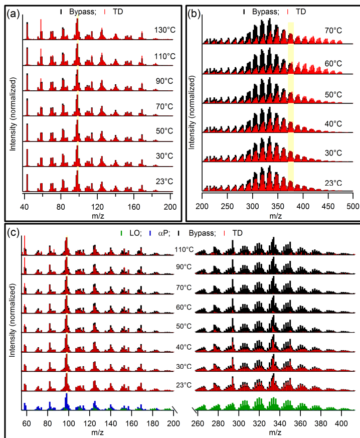
Fig. 2. VUV mass spectra of thermodenuded OA are shown as a function of the thermodenuder temperature (red). The spectrum of the particles through the bypass line is shown for reference (black). (a) Spectra for \alpha P particles, normalized to the peak at m/z = 98 . (b) Spectra for LO particles, normalized to the range m/z = 370\text{--}380 . (c) Spectra for mixed LO + \alpha P particles, normalized to the peak at m/z = 98 . For reference, spectra for \alpha P aerosol (blue) and LO aerosol (green) are shown individually. Note the break in the x-axis and also that the spectral intensity in the right graph ( m/z = 260\text{--}415 ) has been multiplied by a factor of 4 relative to the left graph ( m/z = 55\text{--}200 ).
