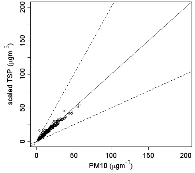
PM10 vs scaled TSP for CHA
