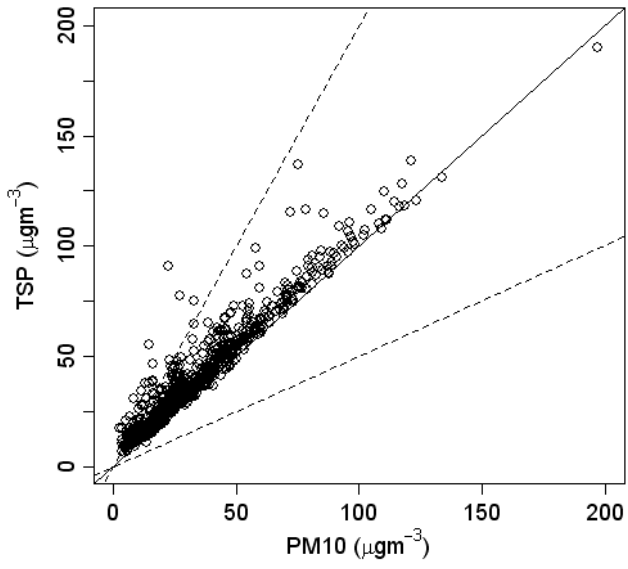
PM10 vs TSP for LUG
