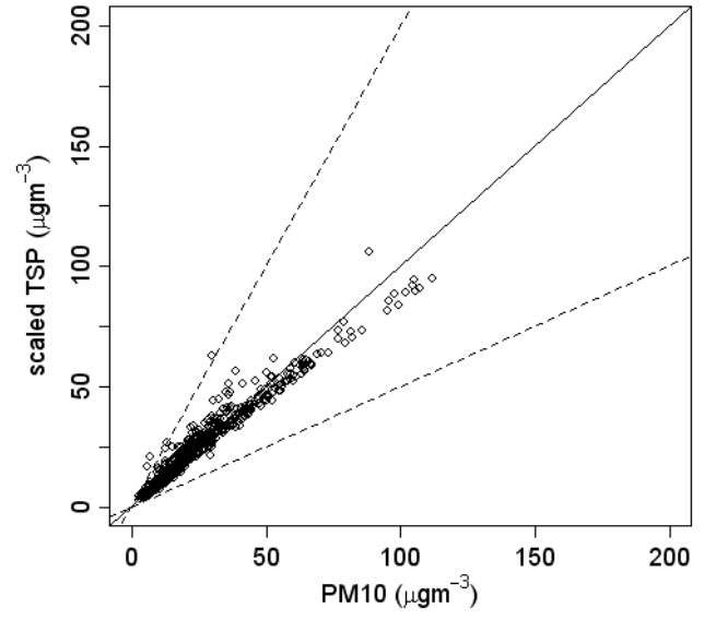
PM10 vs scaled TSP for PAY
