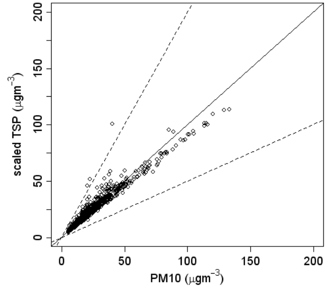
PM10 vs scaled TSP for DUE
