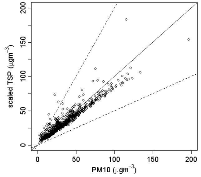
PM10 vs scaled TSP for LUG
