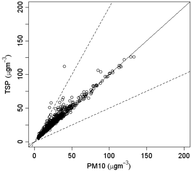
PM10 vs TSP for DUE
