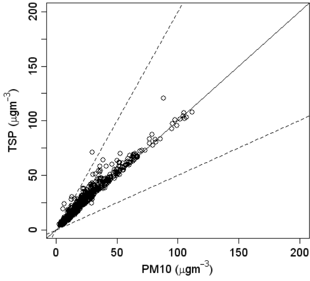
PM10 vs TSP for PAY
