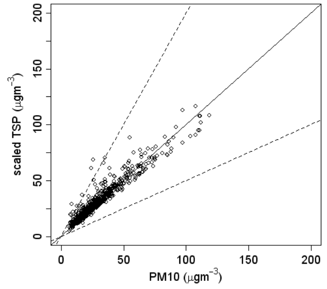
PM10 vs scaled TSP for HAE
