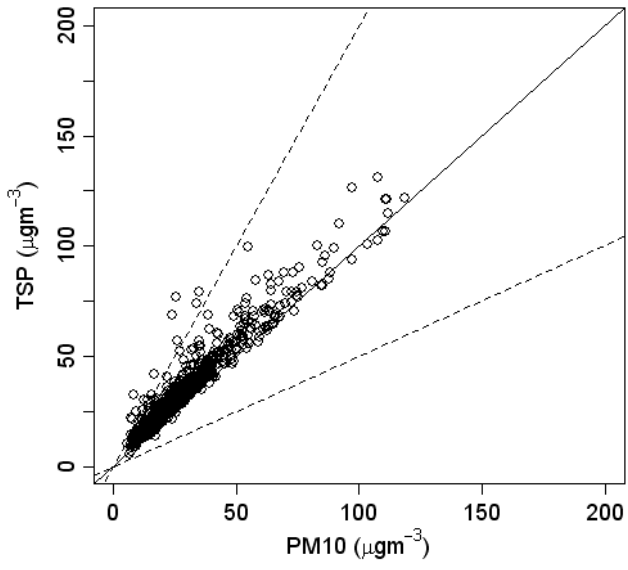
PM10 vs TSP for HAE
