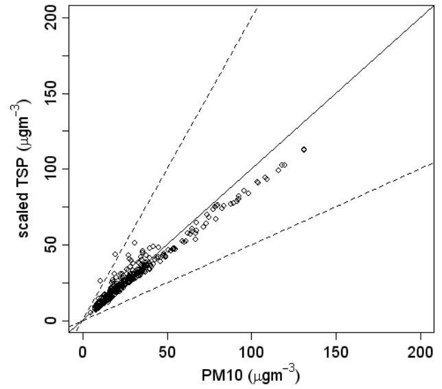
PM10 vs scaled TSP for ZUE
