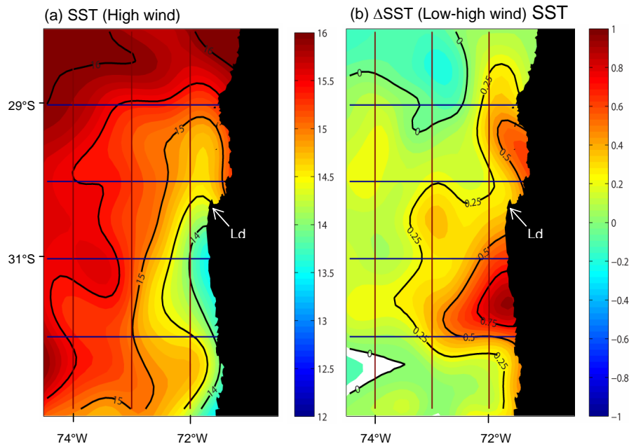
Fig. 7. Sea surface temperature (SST) derived from the Special Sensor Microwave/Imager (SSM/I; see details in Wentz, 1997). (a) Average of SST during the high-wind period (24 November to 2 December 2009). Contours every 0.5^{\circ}\text{C} . (b) SST difference between low-wind days (22 November, 23 November, 3 December, 4 December) minus high-wind period. Contours every 0.25^{\circ}\text{C} . Arrowhead indicates location of point Lengua de Vaca.
