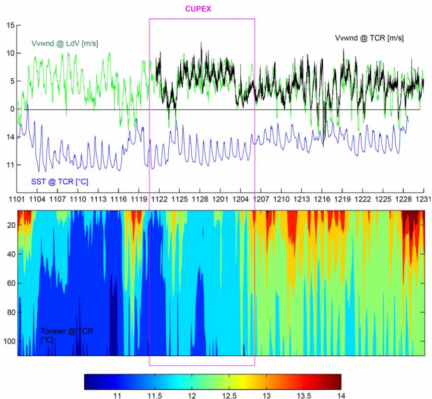
Fig. 9. Lower panel: time-depth section of ocean temperatures (in °C, scale at the bottom; time is indicated in mmdd format in the upper panel) recorded by the mooring 2.2 km off Talcaruca during November–December 2009. The CUPEX period is indicated by the magenta rectangle. The temperature is measured every hour at 5, 10, 15, 20, 25, 30, 40, 50, 70, 90 and 110 m. Upper panel: time series of meridional wind at point Lengua de Vaca (green line) and Talcaruca (black line), and shore SST at Talcaruca (blue line).
