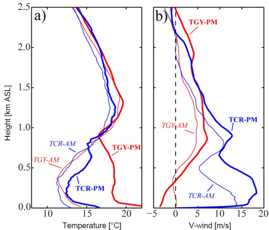
Fig. 14. Morning (08:30 LT, thin lines) and afternoon (17:30 LT, thick lines) mean profiles of (a) air temperature and (b) meridional wind at Talcaruca (blue lines) and Tongoy (red lines). The averages were calculated with the soundings during the CUPeX high-wind period (25 November–2 December 2009).
