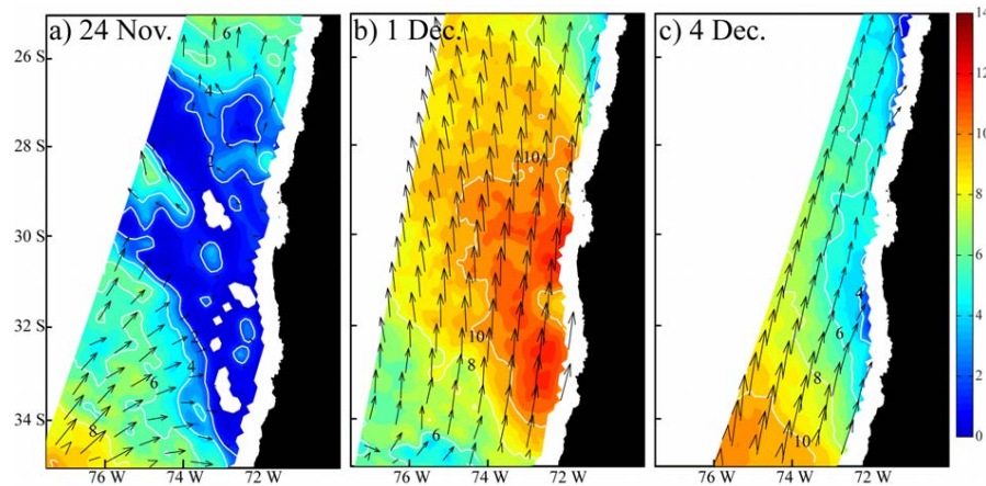
Fig. 5. ASCAT-derived surface wind speed (colours, common scale at right in \text{ms}^{-1} ) and wind vectors (arrows) at 15:00 UTC (11:00 LT) of (a) 24 November, (b) 1 December and (c) 4 December 2009.
