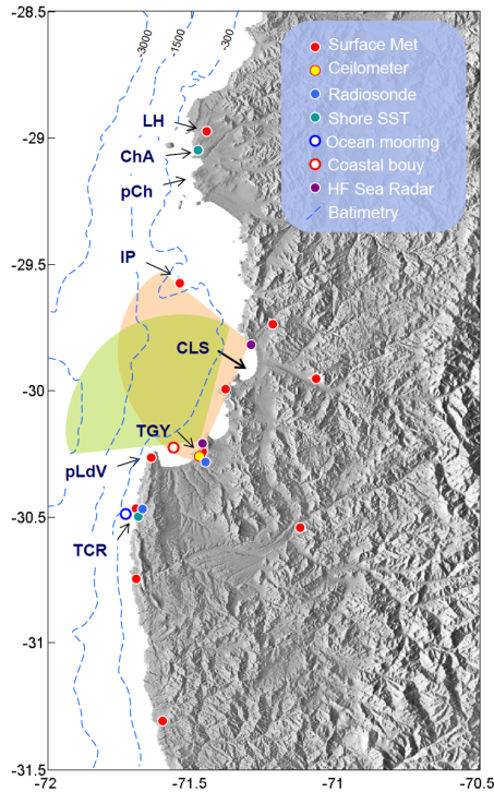
Fig. 2. Shaded relief of the coastal CUPeX area. Coastal mountains are about 500 m high. Relevant locations are TCR = Talcauca, pLdV = point Lengua de Vaca, TGY = Tongoy (town), CLS: Coquimo and La Serena cities, IP = Islote Pajaros, pCh = point Choros, ChA = Chañaral de Aceituno, LH = Loma de Hueso. Also shown is the location of the meteorological and oceanographic measurement systems (color code in the inset). The light orange and green sectors indicate the area covered by the HF Sea Radars at La Serena and Tongoy, respectively. Blue, dashed lines indicate ocean floor depth (in meters).
