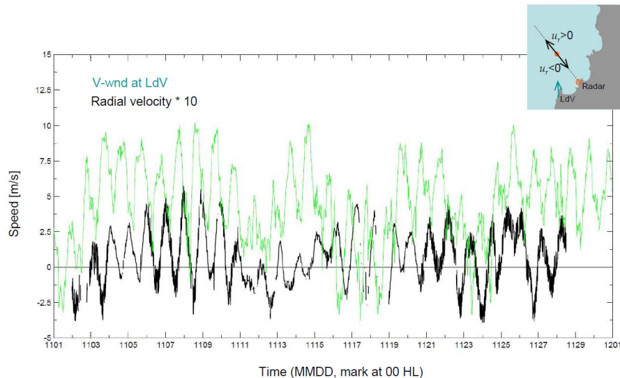
Fig. 13. Radial surface current at 30° S, 71.5° W (black line) measured from the Tongoy HF Radar. Positive (negative) values away from (toward) the radar (see inset). Also shown is the meridional wind speed at point Lengua de Vaca (green line).
