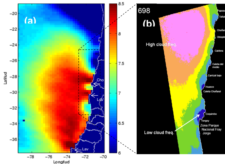
Fig. 3. (a) Spring-Summer (SONDJF) average of surface wind speed derived from 4 years of QuikScat observations. Color scale at right in \text{ms}^{-1} . Note the near coastal jets off points Choros (Ch), Lengua de Vaca (LdV) and Lavapie (Lav). Adapted from Garreaud and Muñoz (2005). (b) Spring (SON) climatology of low cloud frequency derived from visible GOES imagery. Adapted from Gonzalez et al. (2007).
