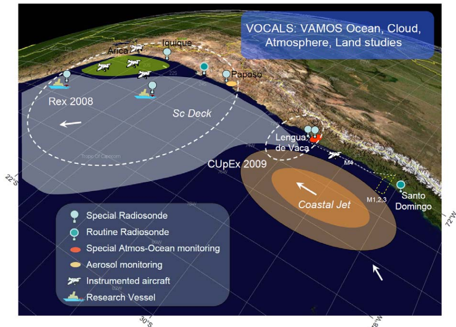
Fig. 1. An overview of the areas targeted by and platforms employed in the VOCALS field experiments. VOCALS-Rex took place in October–November 2008 in a large coastal and open ocean area off southern Perú and northern Chile (down to 25° S), including two research vessels, five fully instrumented aircrafts and one land supersite (Paposo). VOCALS-CUpEx took place in November–December 2009 in the coastal area around 30° S (Lengua de Vaca and the bay of Tongoy) and included 4 research missions off central Chile during 2010 (M1–M4). The map also shows some key locations and atmospheric features over the southeast Pacific: the stratus cloud deck, the coastal low-level jet and the southerly flow around the subtropical anticyclones.
