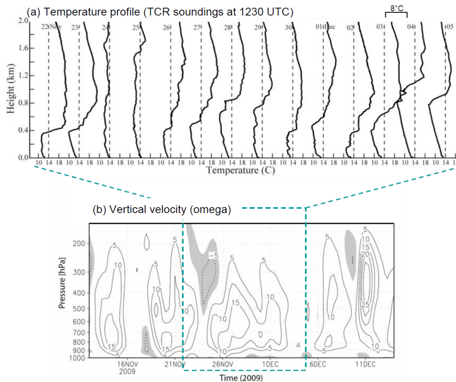
Fig. 10. (a) Vertical profiles of air temperature from the 12:30 UTC (morning) soundings at Talcahuca for each day during CUPeX (dates at the top). The horizontal (temperature) scale is identical for each sounding and the vertical dashed line is the reference 14°C isotherm. (b) Vertical velocity ( \omega -100, contoured every 0.05 hPa/s, shaded area indicates ascending motion) at 30° S, 73° W during November–December 2009. The CUPeX period is indicated by the green box. Data source: NCEP-NCAR reanalysis.
