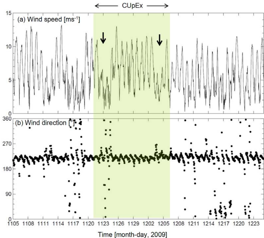
Fig. 4. Half-hourly records of wind speed (upper panel) and wind direction (bottom panel) panel at point Lengua de Vaca during November/December 2009. Central, colored area indicates CUPEX period. The two vertical arrows indicate southerlies relaxation events.
