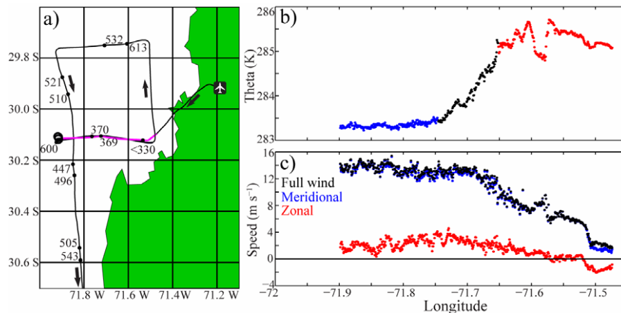
Fig. 15. (a) Trajectory of the BE90 during the flight from La Serena (airport indicated by small plane) to Santiago, as part of the CUPEx research flight 4 (11 July 2010; between 14:45 and 15:20 LT). The flight consisted in constant level legs and porpoising between 300 and 1500 m a.s.l. (5' up and 5' down). The later were used to construct pseudo-vertical profiles of air temperature and humidity. The inversion base was obtained from these profiles and plotted in the map (small numbers in m ASL). (b) and (c) Potential temperature, wind speed and wind components recorded in the constant level (330 m) flight along 30.18° S over the southern Tongoy bay (magenta line in panel a).
