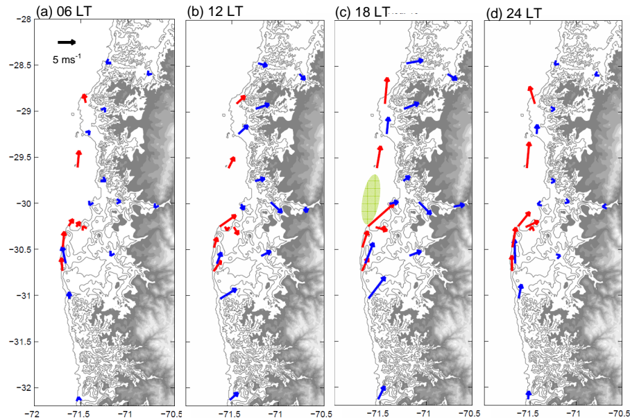
Fig. 12. Mean diurnal cycle of the 10-m winds over the CUPEx area, illustrated by the average wind vectors every 6-h (local time atop of each panel). Red arrows are average winds during CUPEx. Blue arrows are average winds for November/December obtained from different datasets. The green area at 18:00 LT ( c ) indicates the core (wind speed \geq 15 \text{ ms}^{-1} ) of the near-shore coastal jet obtained from a WRF numerical simulation (3 km horizontal resolution) of the CUPEx period described in Rahn et al., 2010. Topographic contours every 250 m, shaded above 1000 m a.s.l.
