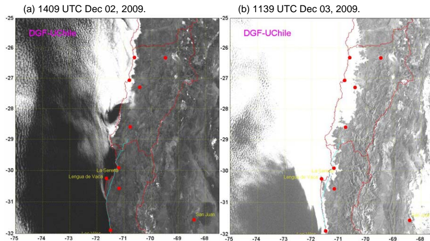
Fig. 11. GOES-13 visible images over the CUpEx area for (a) 14:09 UTC 2 December 2009, and (b) 11:39 UTC 3 December 2009.
