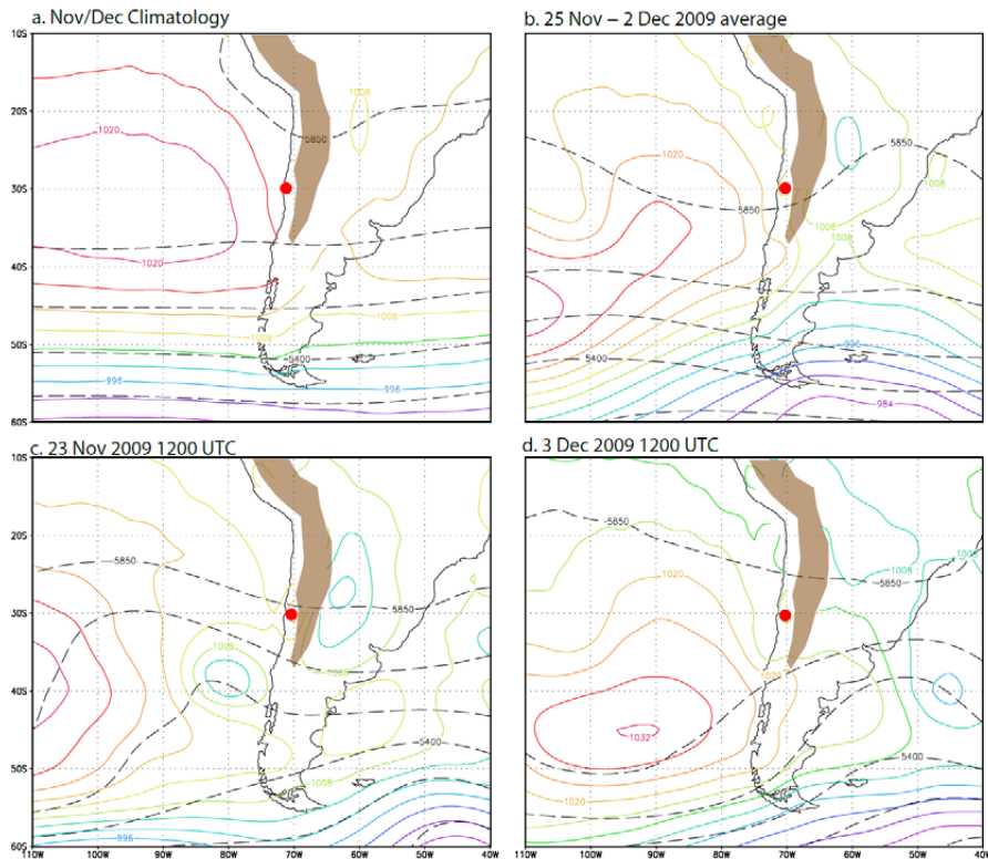
Fig. 6. Daily mean sea level pressure (solid, color lines every 4 hPa) and 500 hPa geopotential height (dashed, black lines every 150 m) for selected dates and periods. Light brown area indicates terrain elevation in excess of 2000 m a.s.l. Red dot indicates Tongoy area. (a) November–December long-term mean. (b) 25 November–2 December 2009 average (high-wind CUpEx period). (c) 23 November 2009 (first southerly wind relaxation during CUpEx, including brief periods of northerlies). (d) 3 December 2009 (second southerly wind relaxation during CUpEx). Data source: NCEP-NCAR reanalysis.
