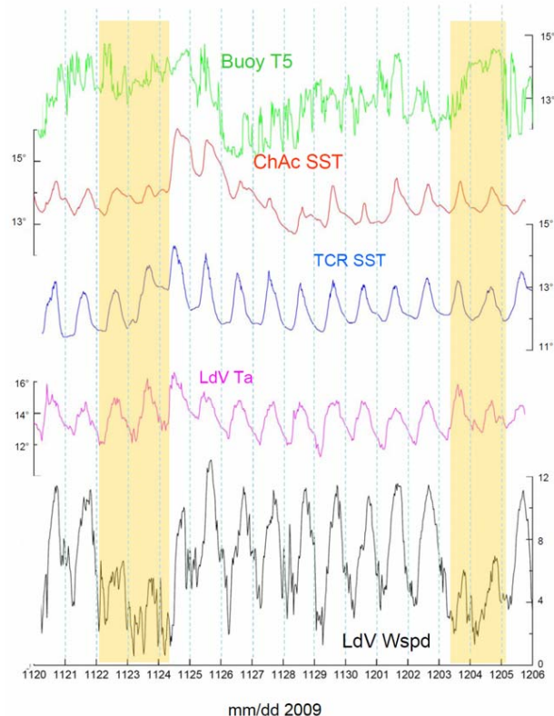
Fig. 8. Times series of selected coastal variables during CUPEx (30-min averages). From bottom to top the variable are: 3.8-m wind speed (black line) and 2-m air temperature (magenta line) at point Lengua de Vaca, shore SST at Talcaruca (TCR, blue line) and Chañaral de Aceituno (ChAc, red line), and 5-m deep sea temperature at the Tongoy bay buoy (green line). The yellow-shaded rectangles indicate the low-wind periods during CUPEx.
