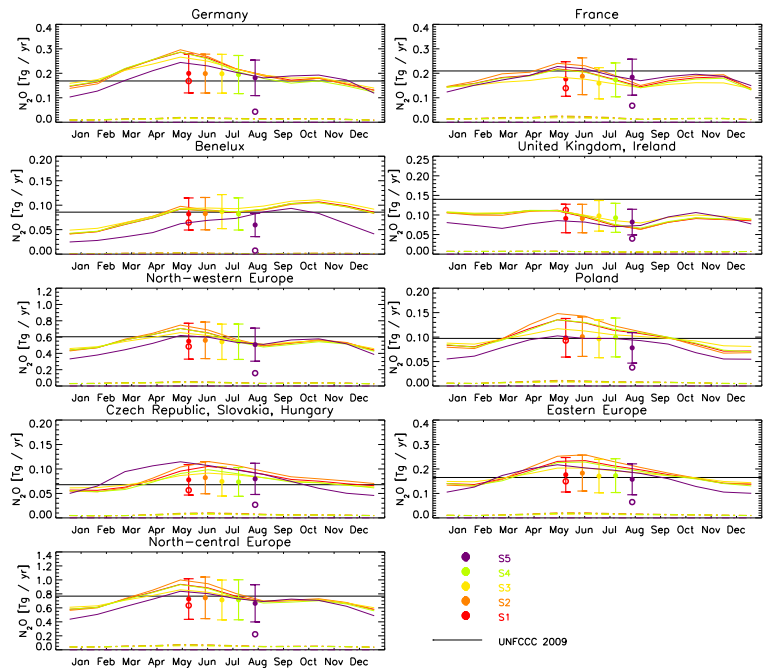
Fig. 5. Total emissions for various northwest European and east European countries for 2006. The filled colored circles represent the results from the 5 inversions and open circles are the applied a priori emissions. The small natural emissions have been subtracted for S1–S4 (while this is not possible for S5, which does not use any detailed a priori knowledge). Emissions reported to UNFCCC are shown by the black solid line (uncertainties of the order of 150% are not shown here, but compiled in Table 5). North-western Europe represents the sum for Germany, France, Benelux, United Kingdom and Ireland, while Eastern Europe represents the sum of Poland, Czech Republic, Slovakia, and Hungary. Finally North-central Europe represents the sum of all considered countries. Colored solid lines represent the seasonal variation of anthropogenic emissions derived in the inversions (3 month running mean), while the colored dash-dotted lines show the small contribution from natural sources.
