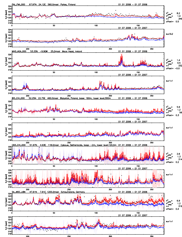
Fig. 2. Time series (days) of observed and simulated N 2 O mixing ratios at 5 of the available European stations: Pallas, Mace Head, Bialystok, Cabauw, and Schauinsland. One year of data, from 1 January to 31 December 2006, is split into two 6-month panels for each station. Blue lines represent a priori simulations and red lines are a posteriori simulations for the reference inversion S1. Shaded areas represent estimated uncertainties of the model simulations. Measurements are shown as black dots. The calculated bias corrections (offset) are given on the right of each panel and have been subtracted from the measurements. Units are ppb.
