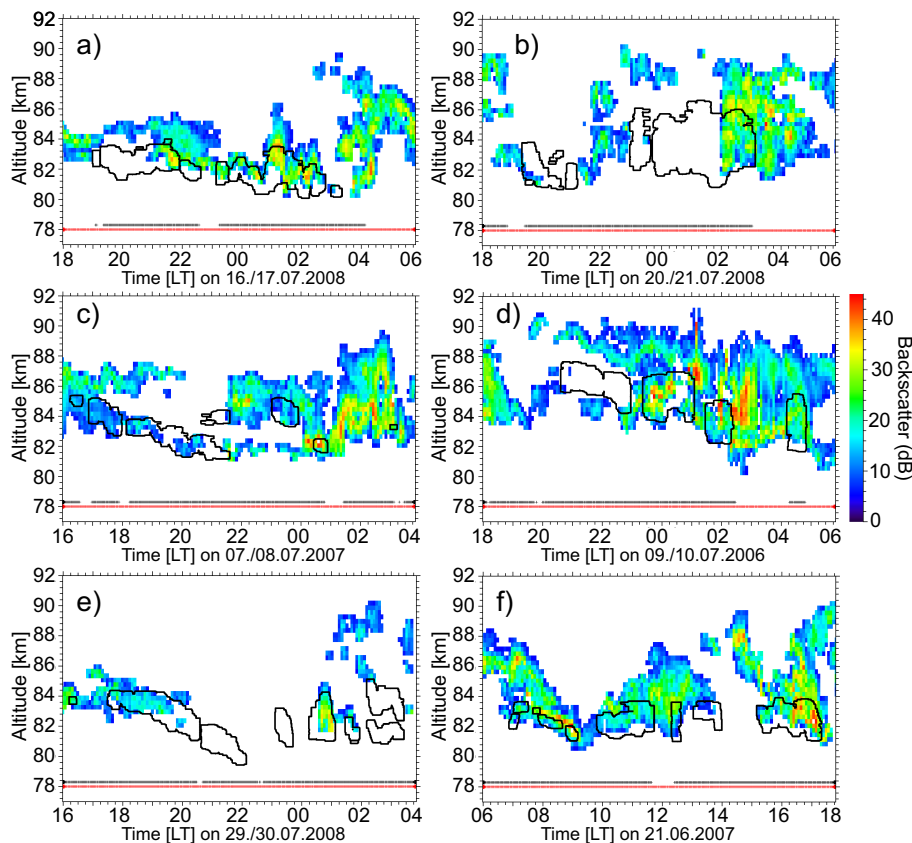
Fig. 2. Examples of joint PMSE (color, limited to >5 dB) and NLC (contour, limited to \beta > \Delta\beta ) observations. Measurement times are indicated by red crosses for radar and in black crosses for lidar.
