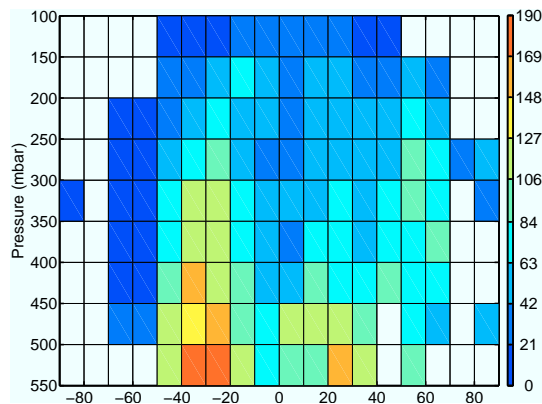
Fig. 6: Average distribution of FA (pptv) measured by ACE-FTS from 2004 to 2008. Measurements are binned in 10^\circ latitude 50 mbar bins. Only bins with more than ten measurements are considered.
