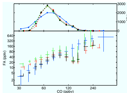
(b) Lower panel: correlation plot between FA and CO (lower panel) for the measurements (blue) and the model: R1 (red), R2b (green), R4 (black). Upper panel: distribution of measured and modeled CO. The extent of the error bars indicate the 25 and 75 percentiles.
