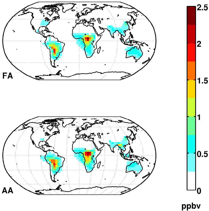
Fig. 1: Annual simulated distribution of FA and AA in the boundary layer.
