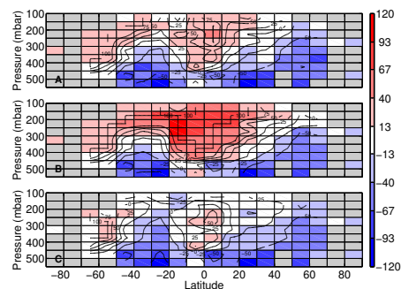
(a) Absolute difference between the model and the ACE-FTS measurement in pptv. Contours indicate the relative difference in % ((model-measurement)/measurement). Cells with no measurements are grayed. Panel A shows the comparison for the reference run (R1), Panel B for R2b and Panel C for R4 (see Sect. 4).
