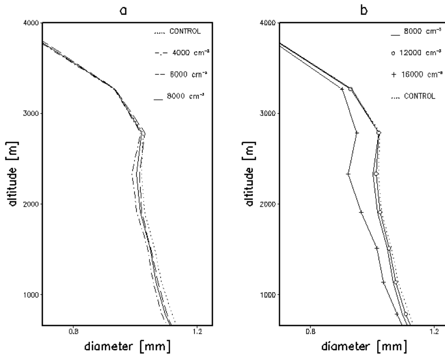
Fig. 12. Idem Fig. 10 but for raindrop mean mass diameters.
