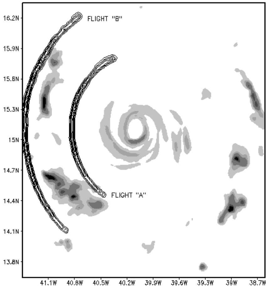
Fig. 1. Virtual flights over internal and external radii. For the combined trajectory, the aircraft would fly north following flight “A” and then south along flight “B”. Black contours denote aircraft flight paths and shaded areas locate convective activity (liquid water path).
