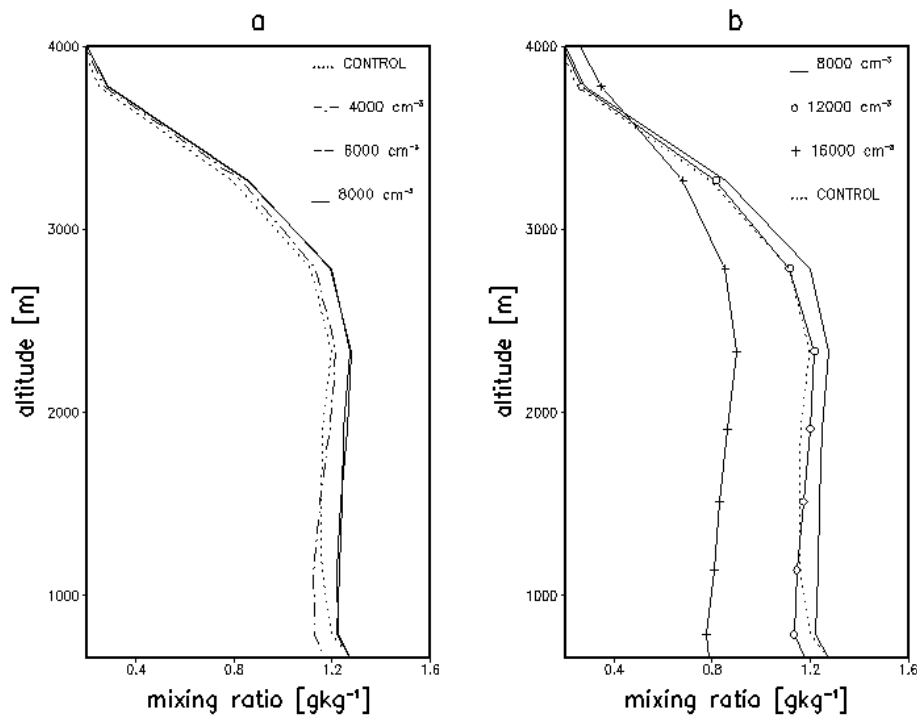
Fig. 11. Idem Fig. 10 but for rain mixing ratio.
