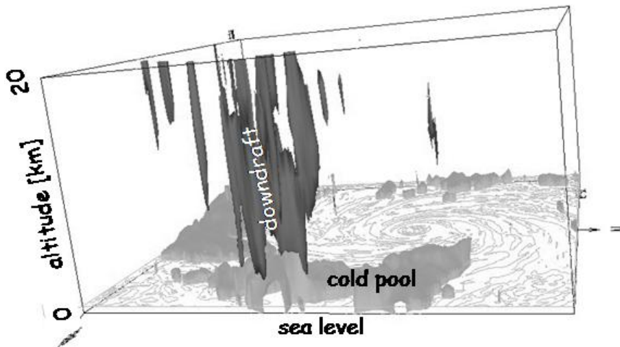
Fig. 9. The largest simulated cold pool and its associated downdraft. The isosurface representing the cold pool (light gray) corresponds to a temperature difference of -4\text{ K} with respect to the horizontal average (for each level). Downdraft isosurface (dark gray) correspond to -2\text{ m s}^{-1} .
