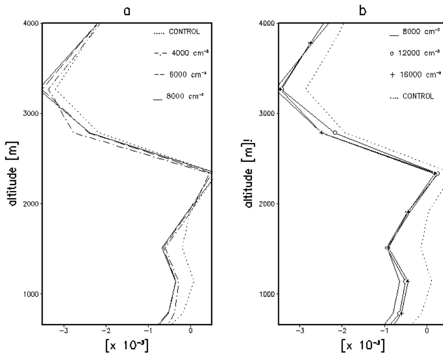
Fig. 10. Comparison of buoyancy within the most intense downdrafts for the control run and the seeded run in panels (a) and (b), respectively.
