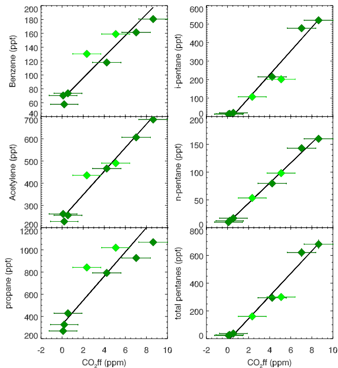
Fig. 5a. Correlations between \text{CO}_2\text{ff} and species measured in the same flasks. Dark and light green symbols are flasks from SAC227 and SAC306 respectively. Lines are the linear regression with errors in both coordinates for flasks from both flights combined.
