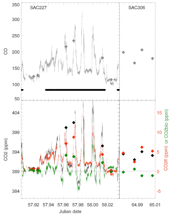
Fig. 7. Top panel: Flask (diamonds) and continuous (lines) measurements of CO from SAC227 and SAC306. The black line indicates times when the aircraft was within the boundary layer. Bottom panel: Flask (diamonds) and continuous (lines) measurements of: total CO 2 (black, left axis); CO 2 ff CO calculated from R_{CO/CO_2ff} and continuous CO (red, right axis); and CO 2 bio calculated as the residual of total CO 2 and CO 2 ff CO (green). Uncertainties are 1 ppb in CO, 0.1 ppm in CO 2 , 1.3 ppm in CO 2 ff and CO 2 bio from flasks, and 0.2–2 ppm in CO 2 ff CO and CO 2 bio from in situ observations.
