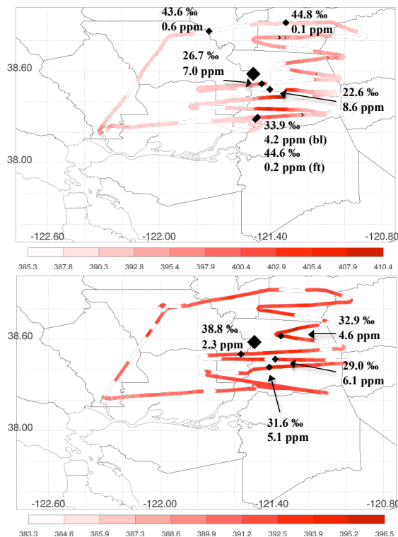
Fig. 1. Flight paths and CO 2 mole fraction (ppm) measured during two flights above Sacramento on 27 February 2009 (SAC227, top) and 6 March 2009 (SAC306, bottom). Black diamonds and numbers indicate the location where each flask was collected and the calculated recently added CO 2 ff mole fraction in that flask. One-sigma uncertainties are 0.1 ppm for in situ CO 2 , and 2.5‰ in Δ 14 CO 2 and 1.3 ppm in CO 2 ff. Large black diamonds indicate the center of Sacramento, thin lines are county boundaries.
