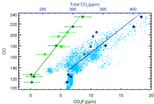
Fig. 2. Correlations between measured CO and CO 2 ff (green points, bottom x-axis) and between measured CO and total CO 2 (blue points, top x-axis). Results from flasks are denoted by large diamonds, with SAC227 in the darker shades and SAC306 in the lighter shades. In situ CO and CO 2 measurements from SAC227 are shown as the small blue points. The lines are the linear regression with errors in both coordinates to the flask data from both flights combined, for CO:CO 2 ff (black line), and CO:CO 2 (grey line). Error bars are the one-sigma uncertainty in CO 2 ff; uncertainties in CO and CO 2 are smaller than the symbol size.
