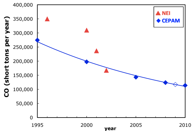
Fig. 4. Inventory-based estimates of CO emissions for Sacramento County, California. Red points are from USEPA NEI county level database ( http://www.epa.gov/ttn/chief/eiinformation.html ). Solid blue points are from the California Air Resources Board CEPAM database ( http://www.arb.ca.gov/ei/ei.htm ). The open blue point is interpolated for 2009 from the fitted curve (blue line) to the CEPAM datapoints.
