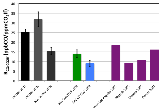
Fig. 3. CO:CO 2ff emission ratios. Gray bars: inventory based emission ratios, from CO and CO 2ff inventories. CO inventories are from the USEPA NEI database from 2002 and 2005 ( http://www.epa.gov/ttn/chief/eiinformation.html ) and California Air Resources Board CEPAM database for 2009 ( http://www.arb.ca.gov/ei/ei.htm ). CO 2ff inventories are from Vulcan (Gurney et al., 2009) and CEPAM (de la Rue du Can, private communication). For each emission ratio, CO 2ff is extrapolated to the same year as the CO inventory. Error bars are derived from the difference between Vulcan and CEPAM CO 2ff inventories. Green: R_{CO/CO_2ff} from this study. Blue: R_{CO/CO_2} from this study (using total CO 2 rather than CO 2ff ). Purple: direct on-road tailpipe emission measurements from Bishop and Stedman (2008).
