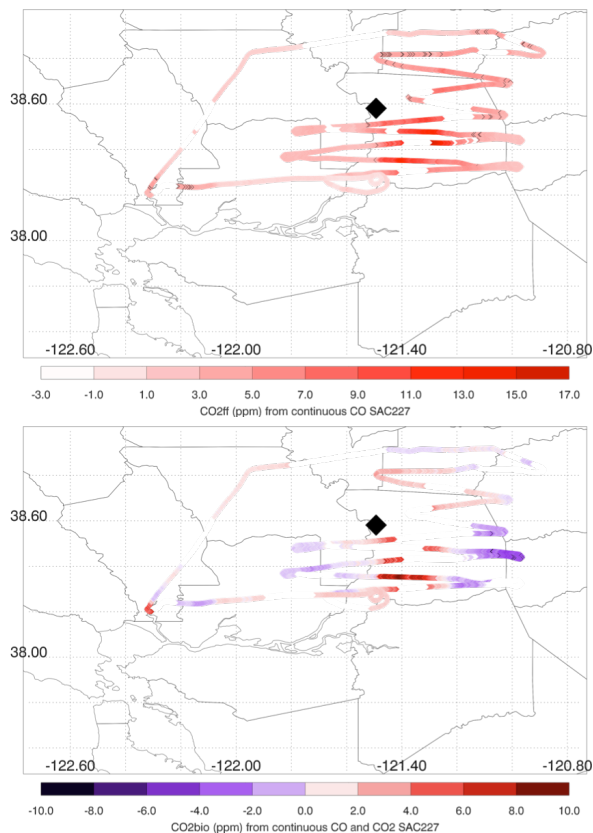
Fig. 8. Continuous \text{CO}_2^{\text{ff}} (top) and \text{CO}_2^{\text{bio}} (bottom) shown as a function of flight path.
