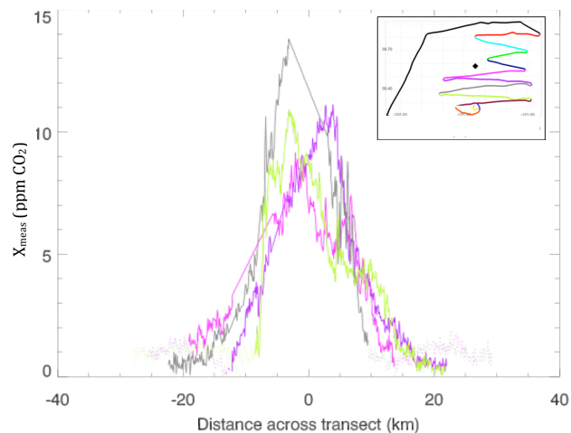
Fig. 9. X_{\text{meas}}(\text{CO}_2^{\text{ffCO}} - \text{background value}) used to integrate for the flux calculation for each of four downwind transects in SAC227. Solid lines indicate the areas inside the plume for each transect. Inset, flight map showing the individual transects.
