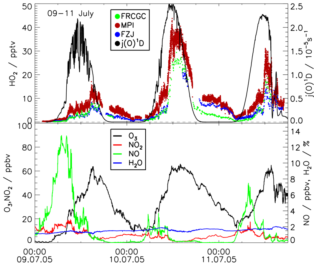
Fig. 2. Time series of HO 2 mixing ratios during ambient air sampling from all instruments at their original time resolution together with the photolysis rate j(\text{O}^1\text{D}) (black line upper panels). In addition, mixing ratios of O 3 (UV absorption photometer), NO 2 and NO (chemiluminescence detector), and water vapor (dewpoint hygrometer) are shown in the lower panels.
