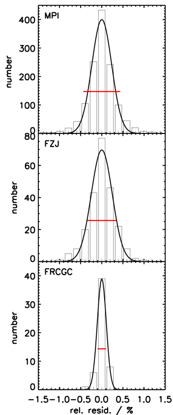
Fig. 5. Frequency distribution of the residuum of a linear fit of measurements on 22 July (1 h periods when HO 2 decreased approximately linearly). The frequency distribution was fitted to a normal distribution (black line). The width agrees with the mean of measurement errors (red line) within the precision of the fit for all instruments.
