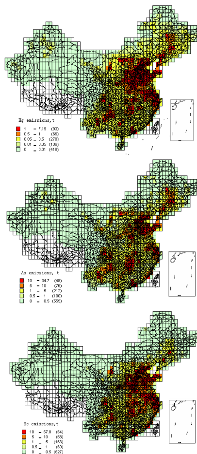
Fig. 7. Gridded total emissions of Hg, As, and Se from coal in China for the year 2005, 1 \times 1 degree (unit: \text{t yr}^{-1} per grid cell).
