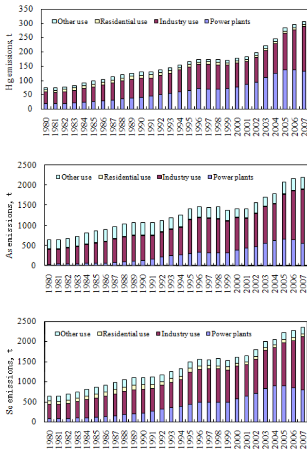
Fig. 4. Trend of Hg, As, and Se emissions by sectors in China, 1980–2007.
