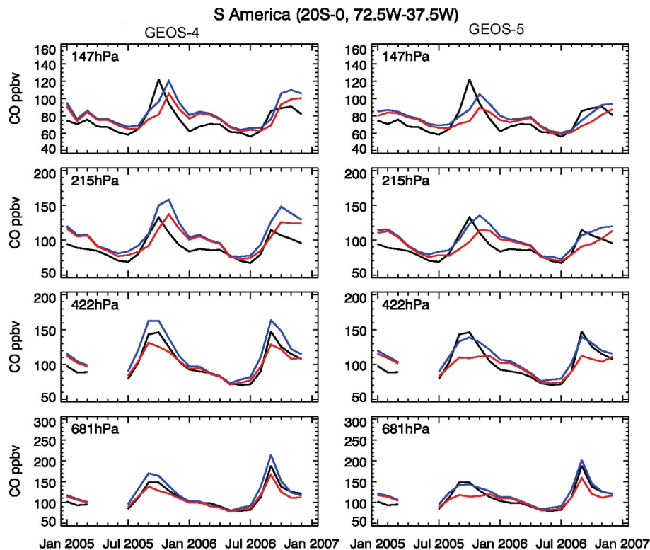
Fig. 14. Time series of TES CO (681 and 422 hPa) and MLS CO (215 and 147 hPa) (black) with (left) GEOS-4, (right) GEOS-5 model results over South America. The standard simulation is in red, and the simulation with adjusted emissions (see text) is in blue.
