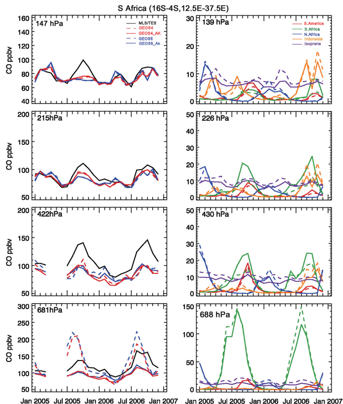
Fig. 17. (Left) Time series of TES CO (681 and 422 hPa) and MLS CO (215 and 147 hPa) (black) and model results for GEOS-4 (red) and GEOS-5 (blue) over southern Africa. Solid lines show the model results with the AKs applied, dashed lines show the model results without the AKs. (Right) Time series of tagged CO tracers over southern Africa from individual sources: biomass burning in South America (red), southern Africa (green), northern Africa (blue) and Indonesia (orange), and the biogenic source from isoprene (purple). See Fig. 8 for further details.
