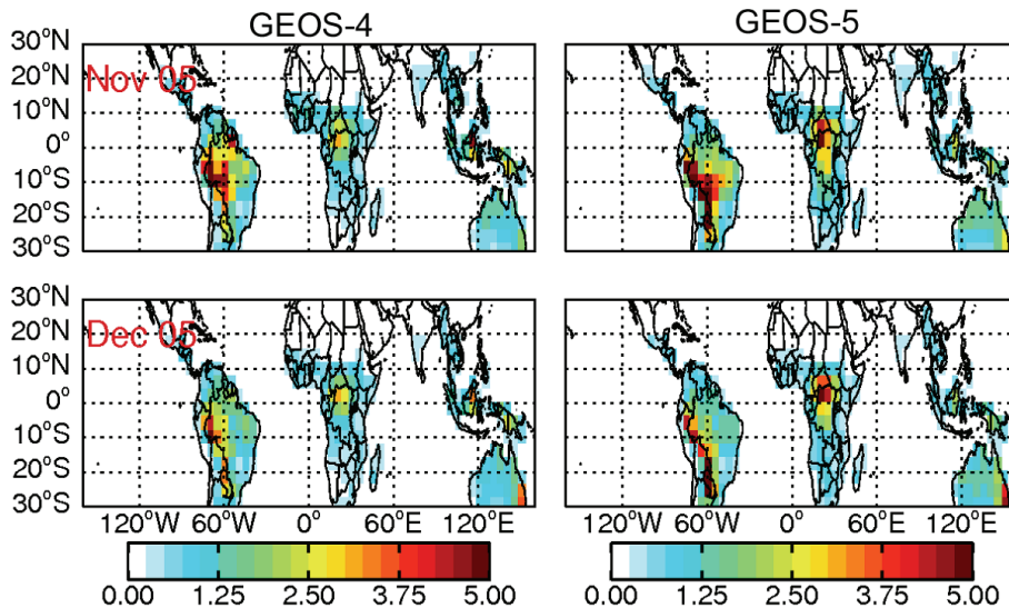
Fig. 13. Isoprene emissions ( 10^{-12} atoms C cm -2 s -1 ) in November (top) and December (bottom) 2005 in the model driven by GEOS-4 (left) and GEOS-5 (right).
