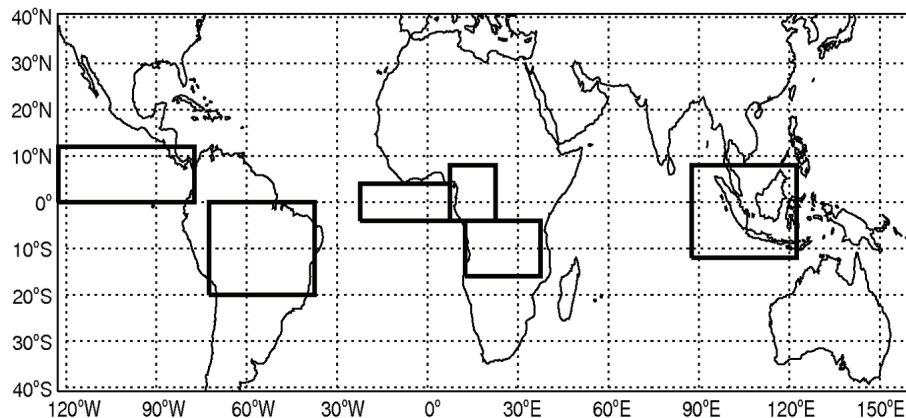
Fig. 7. Location of the regions discussed in this study. From left to right: East Pacific (0–12° N, 122.5–77.5° W), South America (0–20° S, 72.5–37.5° W), Gulf of Guinea (4° S–4° N, 22.5° W–7.5° E), northern Africa (4° S–8° N, 7.5–22.5° E), southern Africa (16–4° S, 12.5–37.5° E) and Indonesia (12° S–8° N, 87.5–122.5° E).
