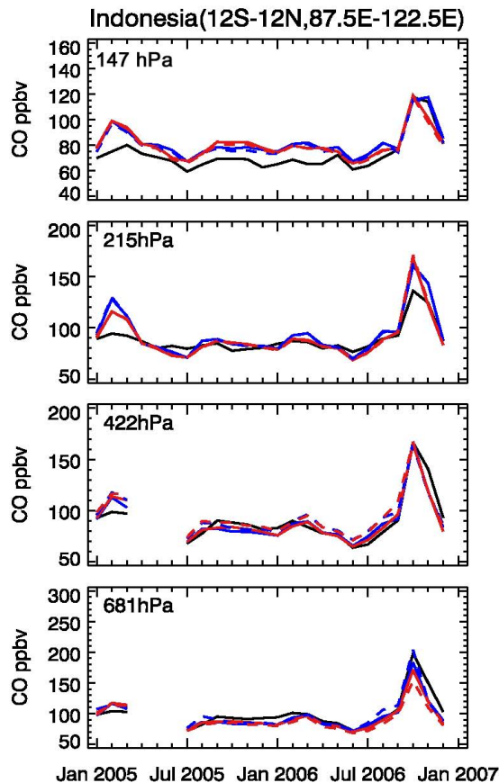
Fig. 25. Time series of TES CO (681 and 422 hPa) and MLS CO (215 and 147 hPa) (black) and model results for GEOS-4 (red) and GEOS-5 (blue) over Indonesia. Solid lines show the model results with the AKs applied, dashed lines show the model results without the AKs.
