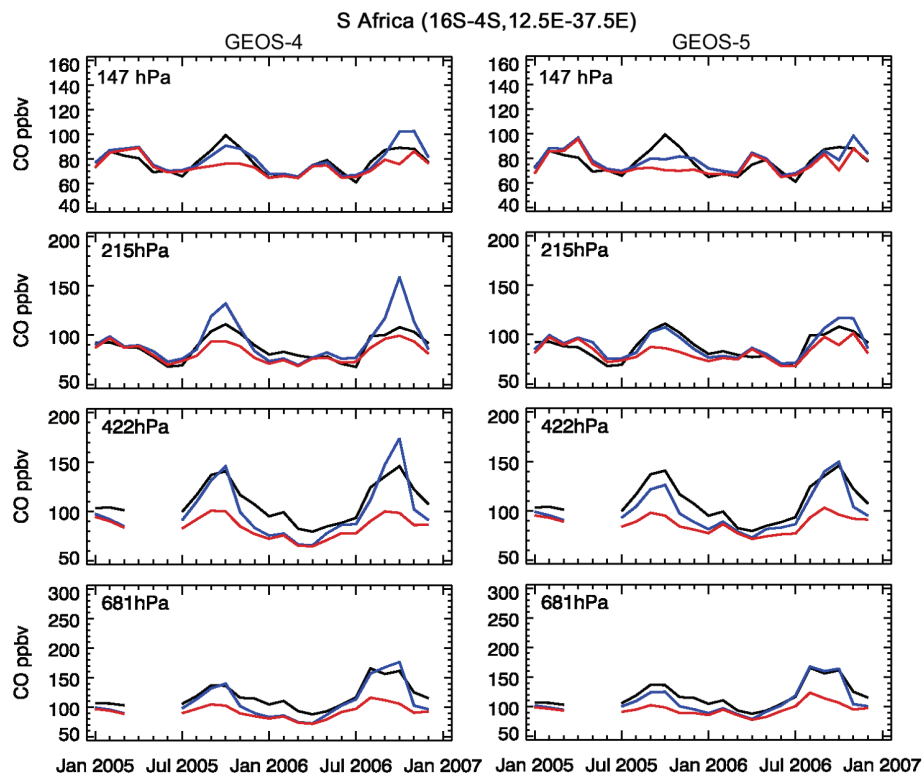
Fig. 20. Time series of TES CO (681 and 422 hPa) and MLS CO (215 and 147 hPa) (black) with (left) GEOS-4, (right) GEOS-5 model results over southern Africa. The standard simulation is in red, and the simulation with adjusted emissions (see text) is in blue. See Fig. 8 for further details.
