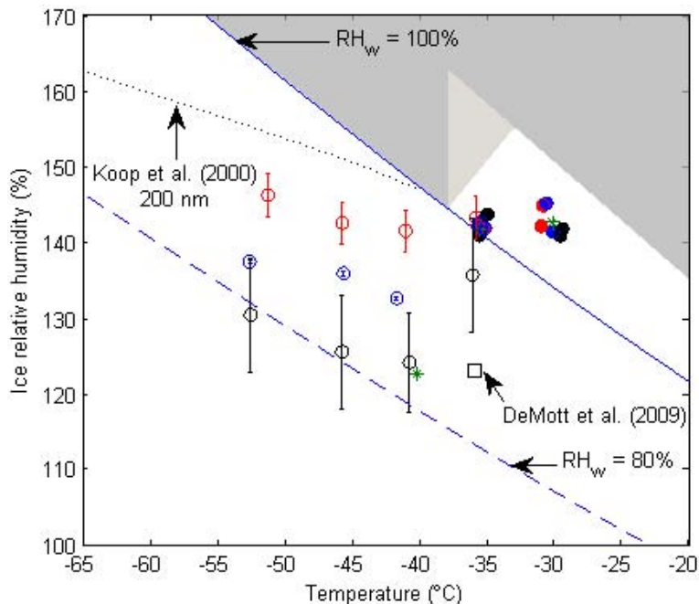
Fig. 2. Conditions for ice nucleation on 5% of CID particles as a function of size: 200 nm (red), 300 nm (blue), 400 nm (black). Open symbols represent data collected with the laboratory unit and filled symbols represent data collected with the aircraft unit. Green stars represent conditions for ice nucleation on 1% of polydisperse CID particles during ICIS. The dark gray shading indicates the region where droplets are known to be counted by the OPC in the CFDC systems. The light gray shading indicates the transition where the state of the particle counted by the OPC is ambiguous. Water saturation, RH_w=80\% and the conditions for which 200 nm (NH_4)_2SO_4 particles nucleate ice according to Koop et al. (2000) are indicated in the figure for reference.
