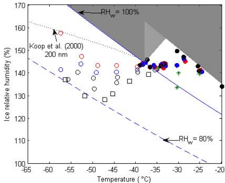
Fig. 3. Conditions for ice nucleation on 5% of SD particles as a function of size: 200 nm (red), 300 nm (blue), 400 nm (black circles) with flow ratios of 7.0:2.5 lpm in the DMA. Black squares are for 600 nm data with flow ratios of 4.0:2.5 lpm in the DMA. Points represent 5% of the particles activating as ice crystals. Open symbols refer to data collected with the laboratory unit, filled symbols refer to data collected in the aircraft unit. Green stars represent conditions for ice nucleation on 1% of polydisperse SD particles during ICIS. The dark gray shading indicates the region where droplets are known to be counted by the OPC in the CFDC systems. The light gray shading indicates the transition where the state of the particle counted by the OPC is ambiguous. Water saturation, RH_w=80\% and the conditions for which 200 nm (NH_4)_2SO_4 particles nucleate ice according to Koop et al. (2000) are indicated in the figure for reference.
