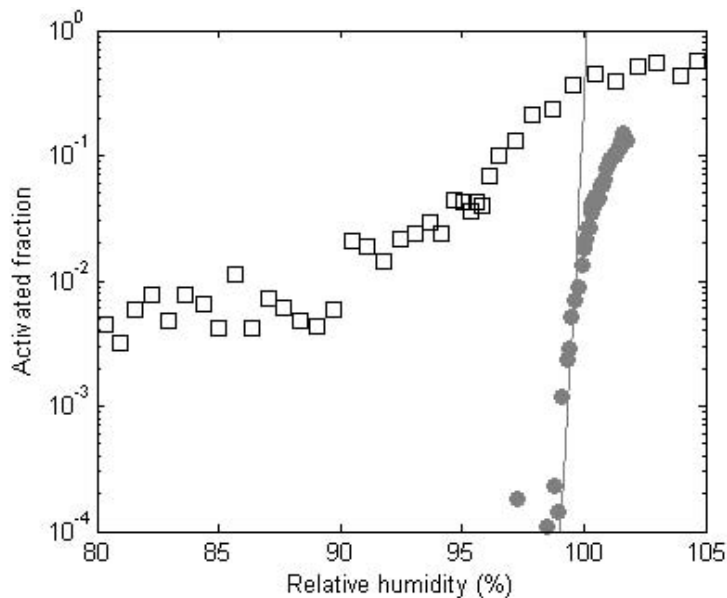
Fig. 6. Activation curves of dry generated 200 nm CID (open squares) and 200 nm ammonium sulfate (filled grey symbols) at -40^{\circ}\text{C} . The solid grey line is the activation of ammonium sulfate predicted by the Koop et al. (2000) parameterization.
