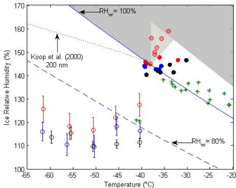
Fig. 1. Conditions for ice nucleation on 1% of ATD particles as a function of size: 200 nm (red), 300 nm (blue), 400 nm (black). Open symbols represent data collected with the laboratory unit and filled symbols represent data collected with the aircraft unit. Green stars represent conditions for ice nucleation on 1% of polydisperse ATD particles during ICIS. The dark gray shading indicates the region where droplets are known to be counted by the OPC in the CFDC systems. The light gray shading indicates the transition where the state of the particle counted by the OPC is ambiguous. Water saturation, RH_w=80\% and the conditions for which 200 nm (NH_4)_2SO_4 particles nucleate ice according to Koop et al. (2000) are indicated in the figure for reference.
