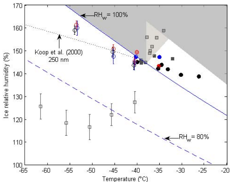
Fig. 4. Conditions for ice nucleation on 1% of SOA-coated ATD particles as a function of size: 160 nm (red), 250 nm (blue), 340 nm (black). Open symbols represent data collected with the laboratory unit and filled symbols represent data collected with the aircraft unit. Conditions for ice nucleation on 1% uncoated 200 nm ATD particles (black squares) are included for reference. The dark gray shading indicates the region where droplets are known to be counted by the OPC in the CFDC systems. The light gray shading indicates the transition where the state of the particle counted by the OPC is ambiguous. Water saturation, RH_w=80\% and the conditions for which 250 nm (NH_4)_2SO_4 particles nucleate ice according to Koop et al. (2000) are indicated in the figure for reference.
