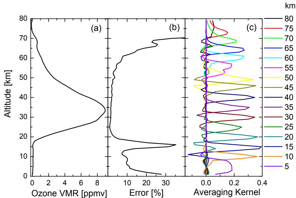
Fig. 8. Ozone VMR profile (panel (a) ) derived from the IASI-MIPAS data fusion and its characterization by means of the percentage retrieval errors (panel (b) ) and of the AKs relative to 5 km step altitudes (panel (c) ).
