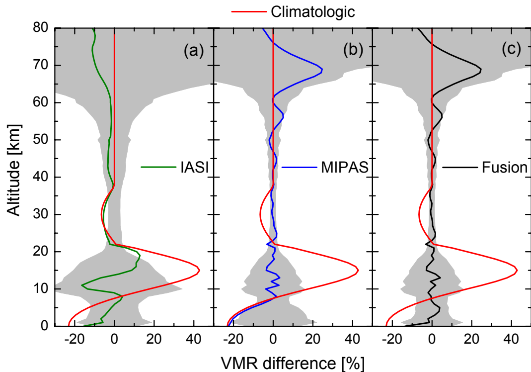
Fig. 2. Percentage differences between the profiles retrieved using only the IASI measurement (green line in panel (a)), only the MIPAS measurement (blue line in panel (b)), the IASI-MIPAS data fusion (black line in panel (c)) and the true profile. The gray areas represent the percentage retrieval errors of the three retrieved profiles. For comparison in all panels the percentage difference between the climatological profile and the true profile is shown (red lines).
