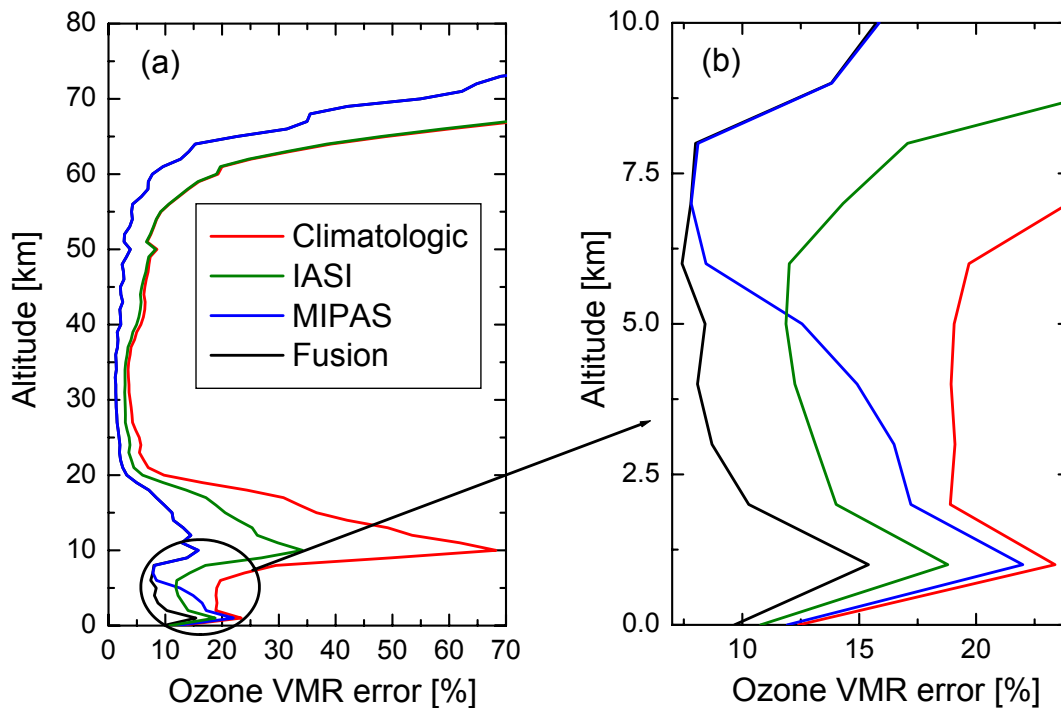
Fig. 3. Percentage retrieval errors for the profiles retrieved using only the IASI measurement (green line), only the MIPAS measurement (blue line) and the IASI-MIPAS data fusion (black line). The standard deviation of the climatological profile (red line) is also reported. Panel (b) shows a blow up of the panel (a) relative to the low atmosphere region.
