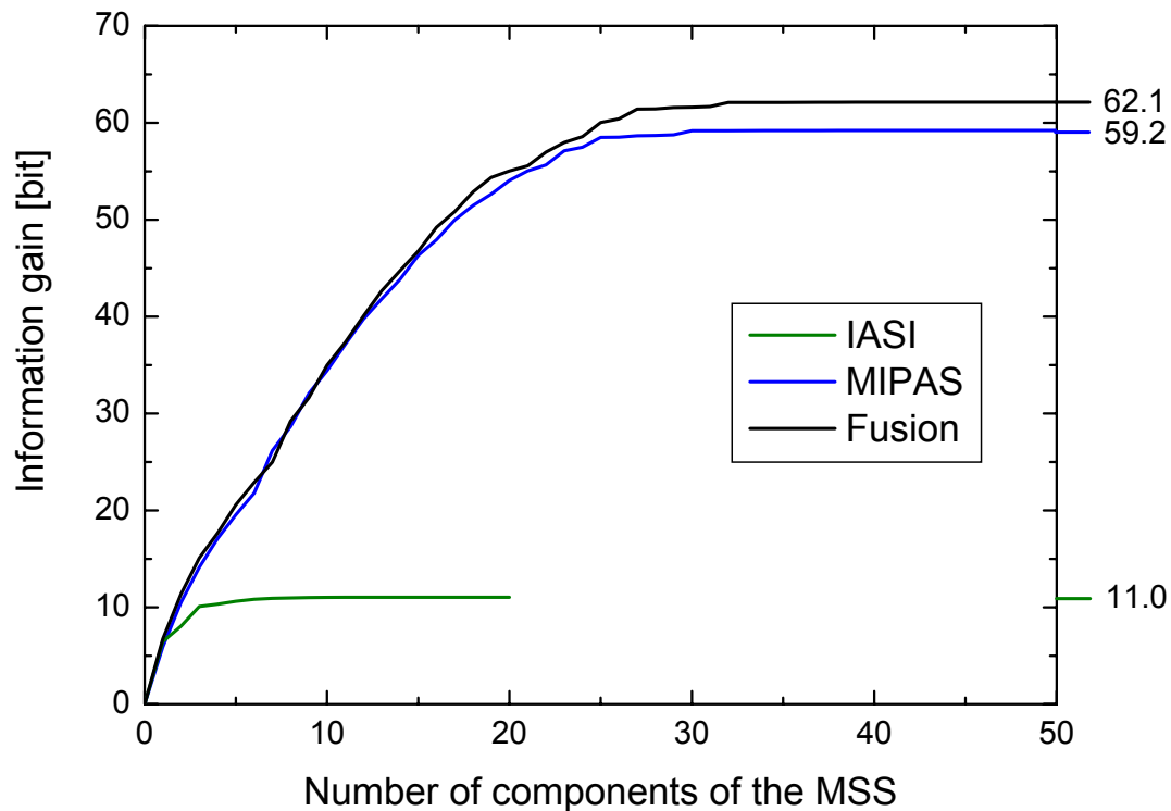
Fig. 6. Information gain as a function of the number of components used to represent the MSS for the profiles retrieved using only the IASI measurement (green line), only the MIPAS measurement (blue line) and the IASI-MIPAS data fusion (black line).
