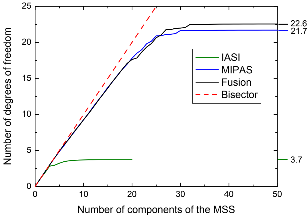
Fig. 7. Number of degrees of freedom as a function of the number of components used to represent the MSS for the profiles retrieved using only the IASI measurement (green line), only the MIPAS measurement (blue line) and the IASI-MIPAS data fusion (black line). The dashed red line corresponds to the ideal case that each measured component contributes with one degree of freedom.
