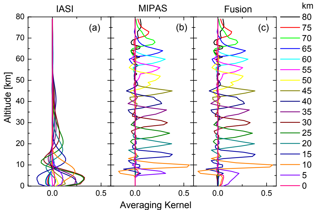
Fig. 4. AKs relative to 5 km step altitudes, in the altitude range 0–80 km, for the profiles retrieved using only the IASI measurement (panel (a) ), only the MIPAS measurement (panel (b) ) and the IASI-MIPAS data fusion (panel (c) ).
