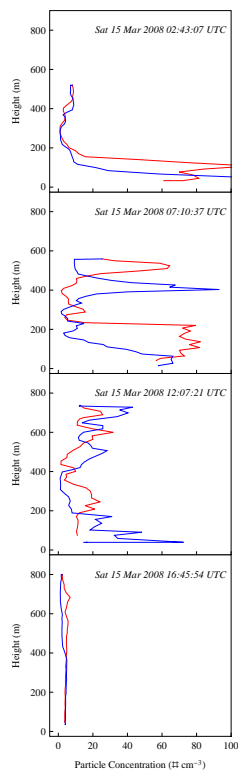
Fig. 10. Vertical profiles of total particle concentration from a four-channel optical particle counter ( 0.3\ \mu\text{m} , 0.5\ \mu\text{m} , 1\ \mu\text{m} , and 5\ \mu\text{m} ) employed in balloon soundings at site K23 on 15 March 2008. Red and blue lines show ascending and descending portions of the soundings.
