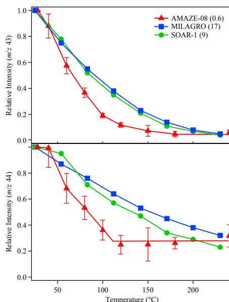
Fig. 13. Thermograms showing the relative signal intensity at m/z 43 ( \text{C}_2\text{H}_3\text{O}^+ ) in the top panel and m/z 44 ( \text{CO}_2^+ ) in the bottom panel for the organic component of the particle mass spectra on 13 March 2008. Signal intensity is for unit mass resolution. The thermograms were corrected for diffusion losses inside the thermodenuder using the approach described by Huffman et al. (2008). The ambient-temperature flow rate through the thermodenuder was 0.6 Lpm. Thermograms for aerosol sampled during the MILAGRO and SOAR campaigns (Huffman et al., 2009b), which represent two polluted megacities, are also included in the figure. The numbers inside the parentheses in the figure legend indicate the organic mass loading ( \mu\text{g m}^{-3} ) of each measurement prior to thermodenuder treatment. The lines in the figure are to guide the eye and do not represent a model fit.
