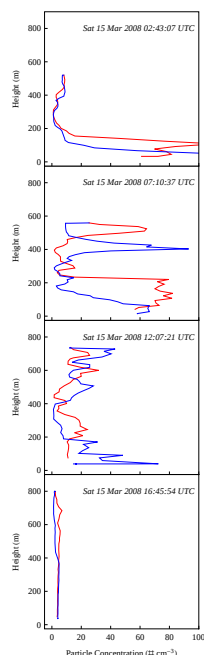
Fig. 10. Vertical profiles of total particle concentration from a four-channel optical particle counter ( 0.3\mu\text{m} , 0.5\mu\text{m} , 1\mu\text{m} , and 5\mu\text{m} ) employed in balloon soundings at site K23 on 15 March 2008. Red and blue lines show ascending and descending portions of the soundings.
