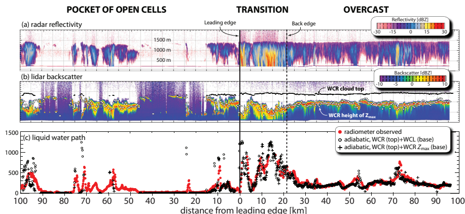
Fig. 12. Time series, from leg SC2 of RF06, of (a) WCR radar reflectivity; (b) WCL lidar backscatter, with WCR cloud top (1 Hz) and the height of the maximum WCR reflectivity (ovals, smoothed with 7 s triangular filter and plotted every fifth point for clarity) overlaid; (c) liquid water path from the microwave radiometer (red circles) and estimated using two adiabatic models. Both models use the WCR observed cloud top height, but one uses the lidar-derived cloud base height where available (open circles), and the other uses the height of the maximum WCR radar reflectivity as a proxy for the cloud base height (crosses) where strong drizzle precludes accurate WCL cloud base height estimates.
