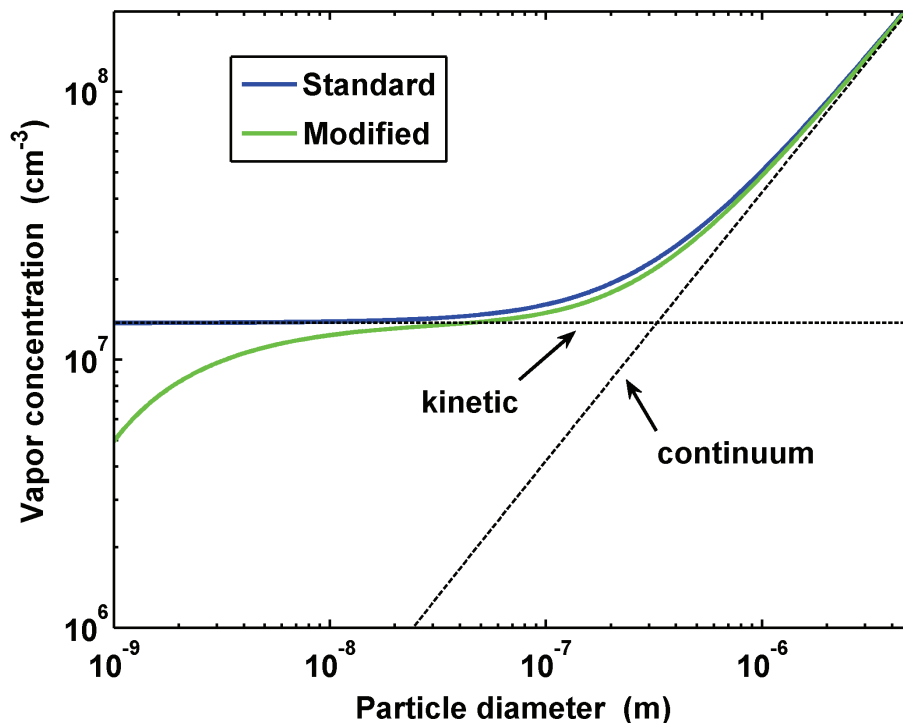
Fig. 2. Vapor concentration required for growth rate of 1 nm/h as function of particle diameter. Vapor is assumed to have molecular properties of sulphuric acid (molecule mass 98 amu and liquid phase density 1.83 g cm -3 ) and negligible saturation vapor pressure. “Modified” refers to the method of this study and “standard” to the Fuchs-Sutugin approach. Dashed lines show the kinetic (or free-molecular) and continuum regime results.
