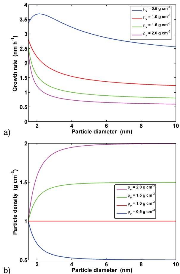
Fig. 5. (a) Particle growth rate as function of diameter in the case when the density of the particle changes due the condensation of vapor. (b) Density of the particle as function of diameter. The density of the initial 1.5 nm diameter particle is 1.0 \text{ g cm}^{-3} .
