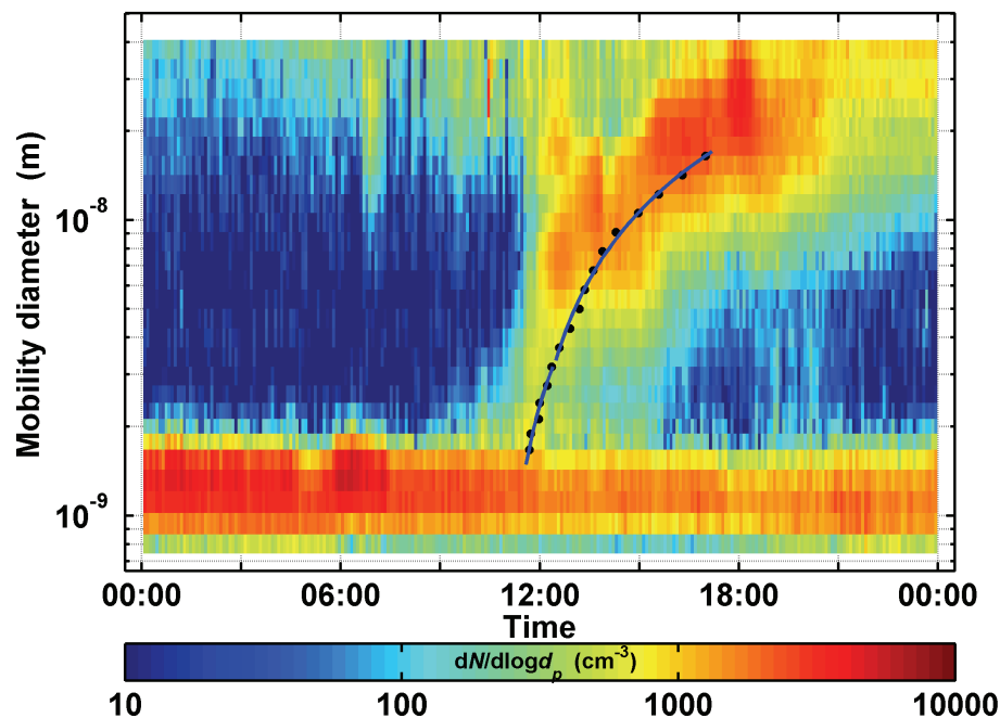
Fig. 9. Size spectra of negative air ions measured at Hyytiälä on 5 May 2007. Black dots represent locations of maxima of number concentrations in each size bin of the instrument. The solid line is a linear fit to those points. Growth rate of the particles is 2.1 nm/h in size range 1.5 to 3 nm, and 2.9 nm/h from 3 to 20 nm.
