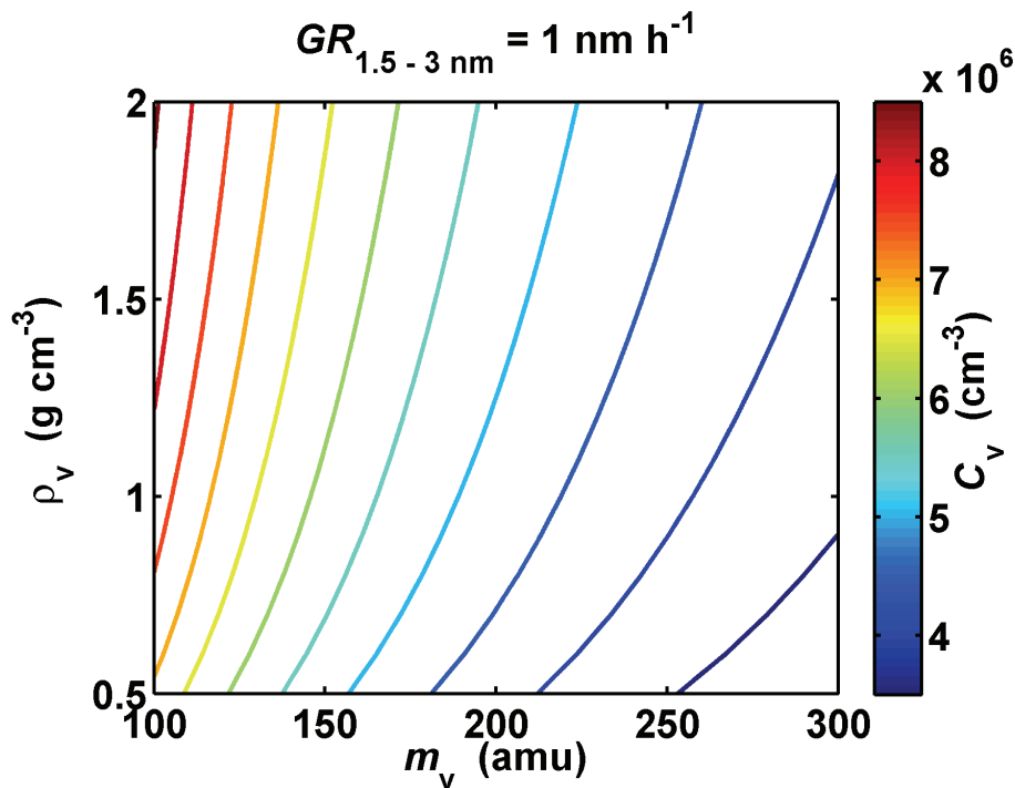
Fig. 6. Variation of the vapor concentration required for growth rate 1 \text{ nm h}^{-1} over 1.5–3 nm size range as function of vapor molecule mass m_v and liquid phase density \rho_v .
