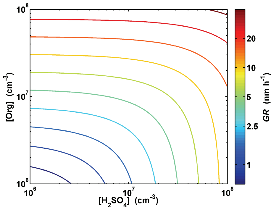
Fig. 7. Particle growth rate “GR” over 1.5–3 nm size range as function of sulphuric acid and organic vapor concentration, assuming GR = GR_{H_2SO_4} + GR_{org} . Organic vapor molecule mass is 300 amu and liquid phase density 0.5 \text{ g cm}^{-3} .
