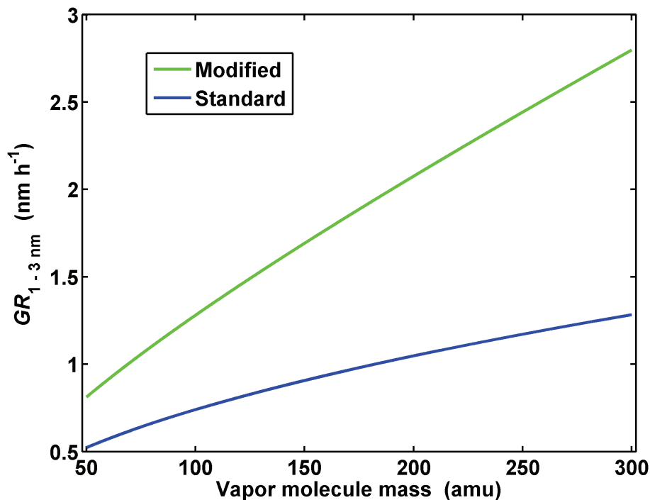
Fig. 3. Particle growth rate over 1–3 nm diameter range as function of condensing vapor molecule mass. Vapor concentration is 10^7 \text{ cm}^{-3} . “Modified” refers to the method of this study and “standard” to the Fuchs-Sutugin approach.
