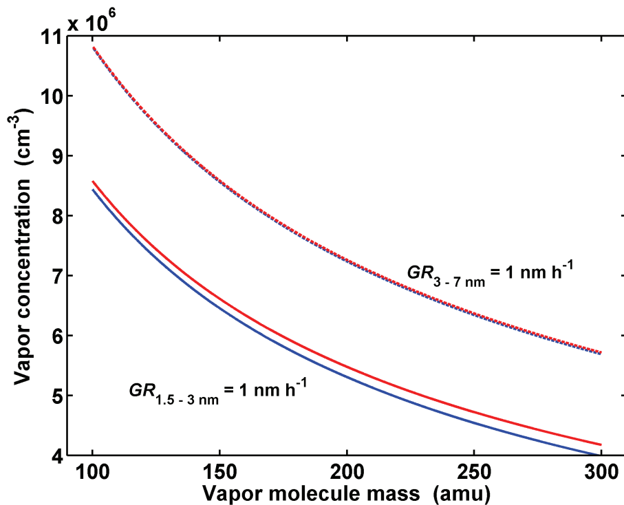
Fig. 1. The required vapor concentration for growth rate 1 \text{ nm h}^{-1} over particle size range 1.5–3 nm (solid lines) and 3–7 nm (dashed lines). Result using approximation of Eq. (11) is shown in red and result by numerically integrating Eq. (9) is shown in blue.
