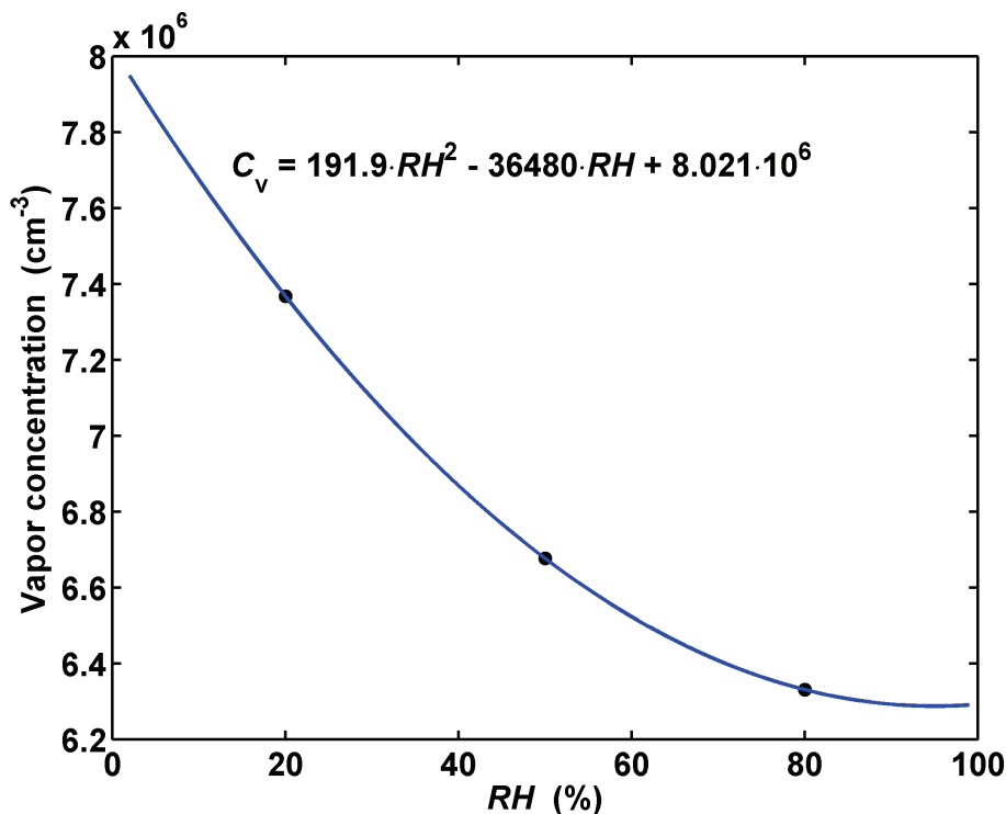
Fig. 8. Concentration of hydrated sulphuric acid required for growth rate 1 \text{ nm h}^{-1} over size range 1.5–3 nm as a function of relative humidity. Points represent the calculated sulphuric acid concentrations according to Eq. (12), when the relative humidity dependent hydration of sulphuric acid molecules has been taken into account. Solid line is a second order polynomial fit to the calculated points. In the fitting equation RH is given in percents.
