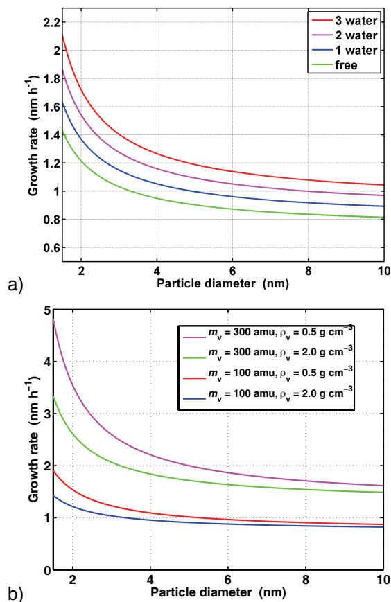
Fig. 4. Particle growth rate according to Eq. (9) as function of particle size and molecular properties of the condensing vapor. Vapor concentration is 10^7 cm -3 , and saturation vapor pressure is negligible. In (a), free sulphuric acid and hydrated molecules with one, two or three water molecules.
