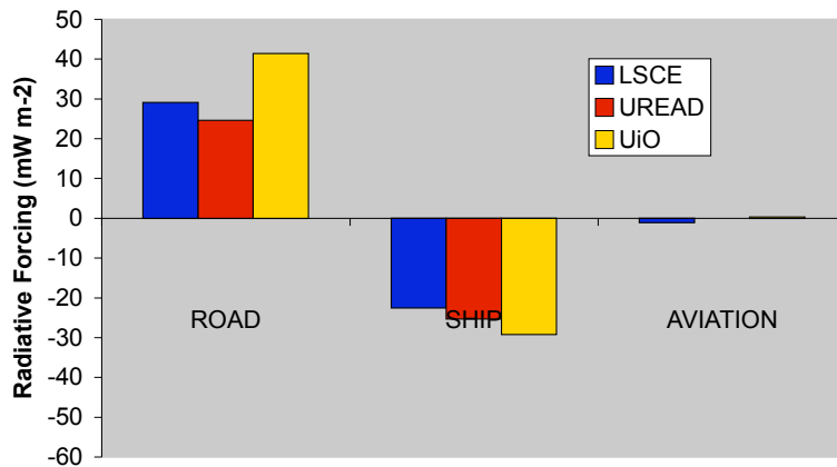
Fig. 5. Comparison of the total direct aerosol global-mean radiative forcings ( \text{mW m}^{-2} ) for the three sub-sectors. For all three models, the BC aerosols are considered internally mixed.
