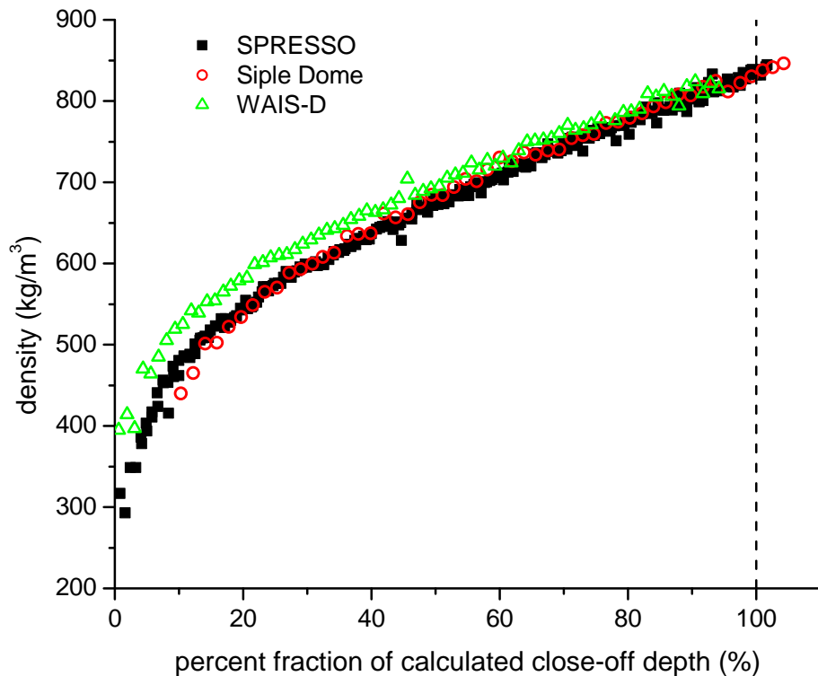
Fig. 4. Ice density for SPRESSO (black squares), Siple Dome (red circles), and WAIS-D (green triangles) cores. The x -axis is a normalized depth scale calculated by dividing the depth of density measurements by the firn close-off depth calculated from Eq. (1) (surface at 0%). The dashed line indicates full close-off as predicted by this equation. The density data extend to the actual depth, at which the deepest firn sample at each individual site was collected.
